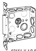
52151-V-1/2 & 3/4 "SV" Bracket mounted flush
