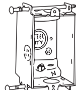
A-257-25 With nails slanted for easy drive-in
