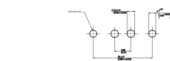
Shell Size E Contact Arrangement 2W2/2WK2 No. of Size 20 Cavities 0 #20 No. of Size 8 Cavities 2 #8
