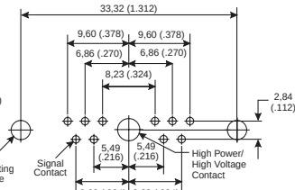
Shell Size A Contact Arrangement 11W1 No. of Size 20 Cavities 10 #20 No. of Size 8 Cavities 1 #8
