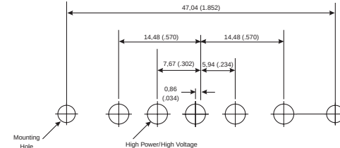
Shell Size B Contact Arrangement 5W5 No. of Size 20 Cavities 0 #20 No. of Size 8 Cavities 5 #8
