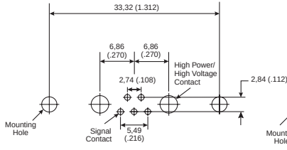
Shell Size A Contact Arrangement 7W2 No. of Size 20 Cavities 5 #20 No. of Size 8 Cavities 2 #8
