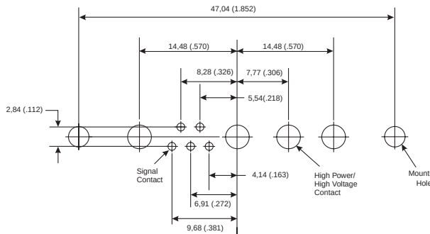
Shell Size B Contact Arrangement 9W4 No. of Size 20 Cavities 5 #20 No. of Size 8 Cavities 4 #8
