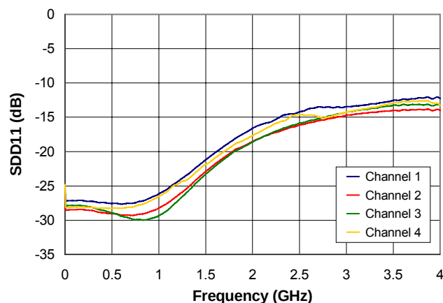
FIGURE 13. INPUT DIFFERENTIAL RETURN LOSS
