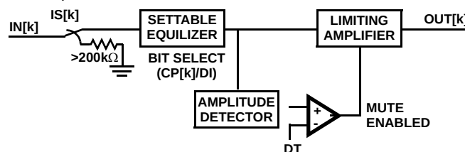
FIGURE 17. FUNCTIONAL DIAGRAM OF A SINGLE CHANNEL WITHIN THE QLx4300-S45
