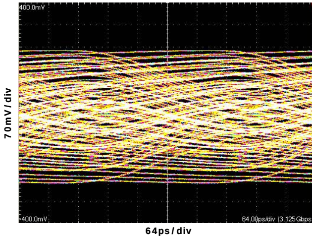
FIGURE 7. RECEIVED SIGNAL AFTER 20m OF 26AWG TWIN-AXIAL CABLE, 3.125Gb/s
