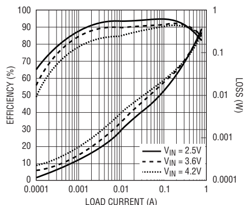
Efficiency and Loss vs Load Current
