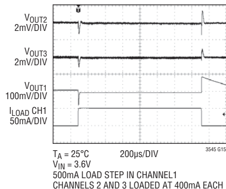
Load Step Crosstalk
