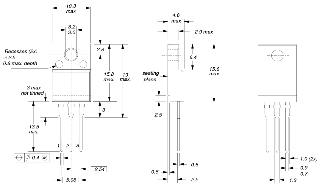
Fig.13. SOT186A; The seating plane is electrically isolated from all terminals.
