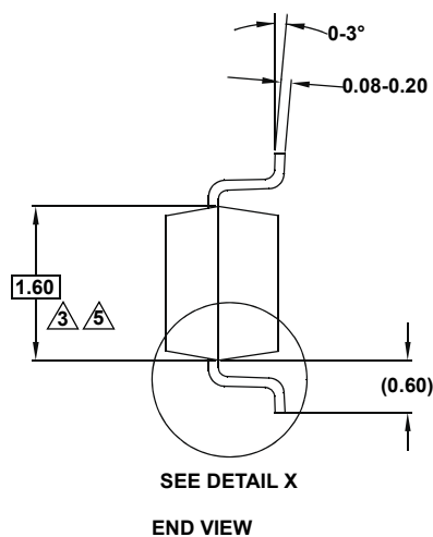
END VIEW
