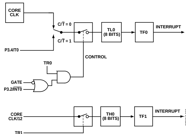
Figure 69. Timer/Counter 0, Mode 3
