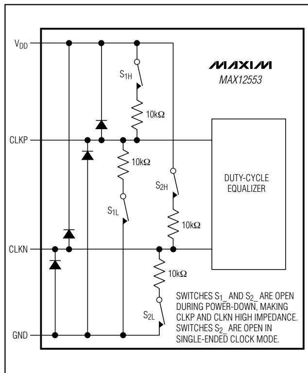
Figure 5. Simplified Clock-Input Circuit
