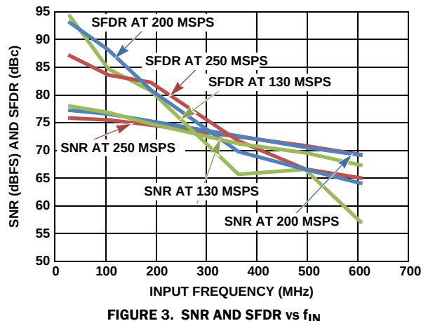
FIGURE 3. SNR AND SFDR vs f_{IN}
