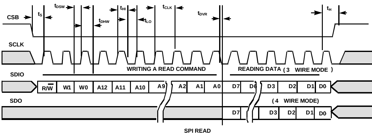
SPI READ
