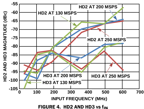
FIGURE 4. HD2 AND HD3 vs f_{IN}
