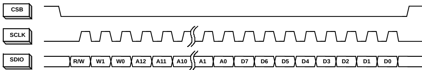
FIGURE 42. MSB-FIRST ADDRESSING
