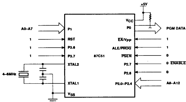
Figure 14. Program Verification
