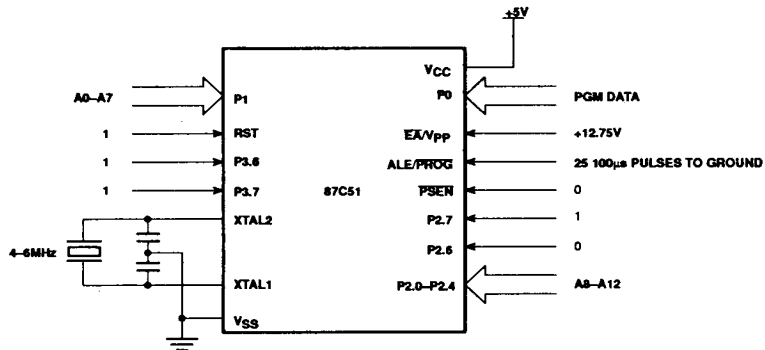
Figure 12. Programming Configuration
