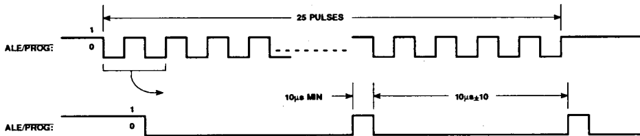
Figure 13. PROG Waveform
