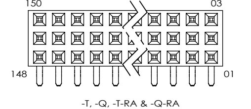
FIG 3 POLARIZATION LOCATION (INSERT PK-06-N INTO SPECIFIED POSITION & BREAK OFF TAB) (-RA OPTION SHOWN FOR ORIENTATION PURPOSE ONLY)
