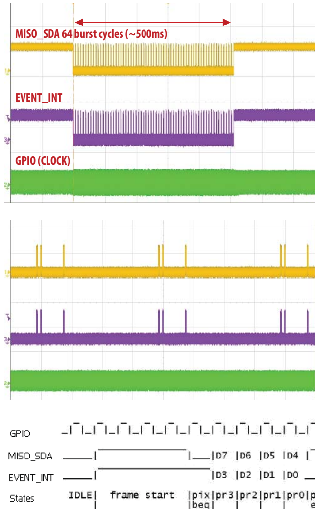
Figure 9. Signals for frame start
