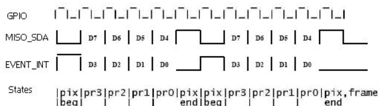
Figure 10. Frame End
