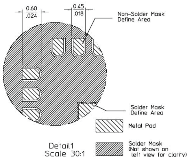
Figure 3c. Recommended Customer's PCB PADOUT and spacing
