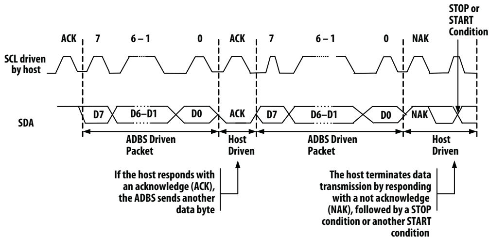
Figure 21. Sensor packets
