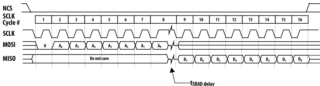
Figure 13. Read Operation
