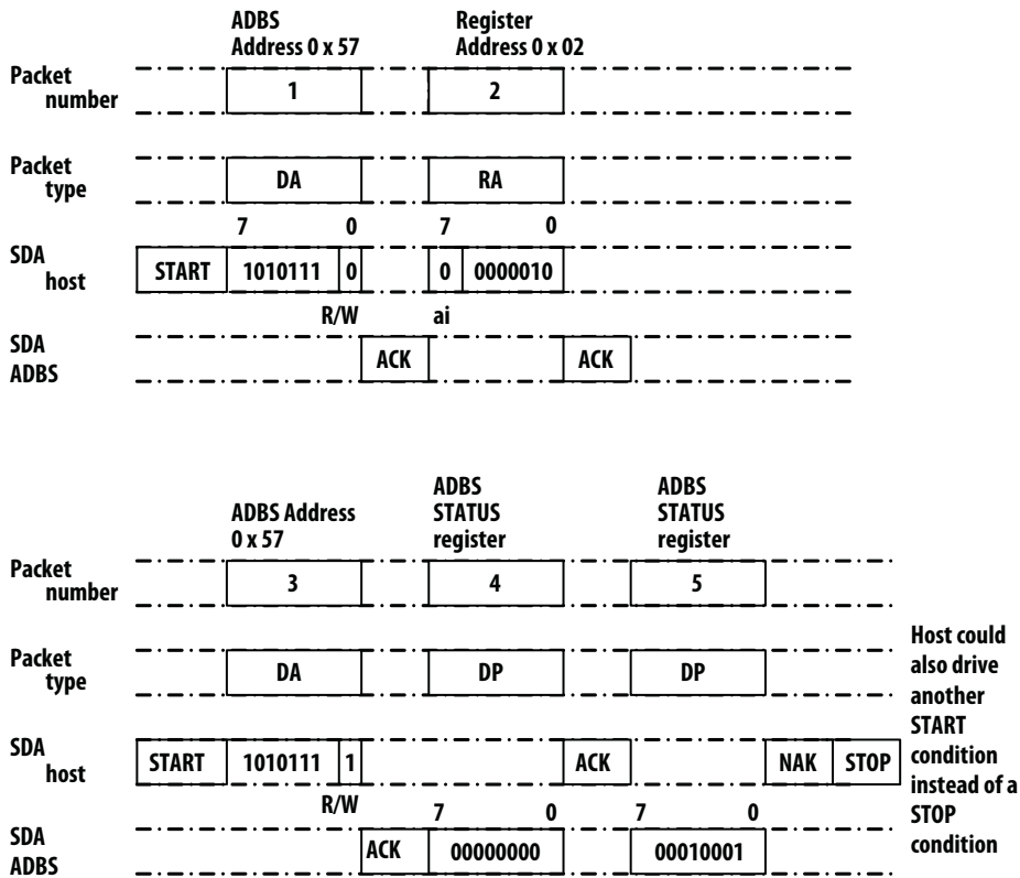
Figure 24. TWI polling
