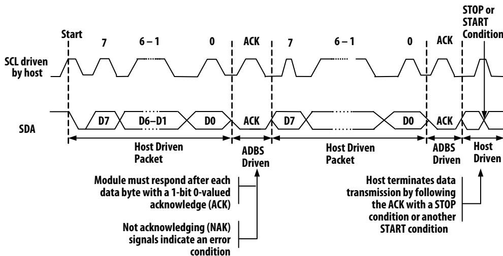
Figure 20. Host packets
