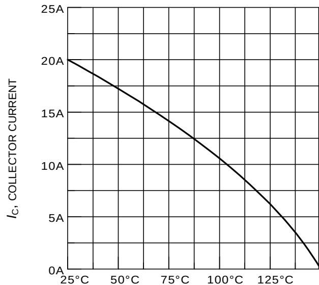
Figure 4. Collector current as a function of case temperature ( V_{GE} \leq 15\text{V} , T_i \leq 150^\circ\text{C} )
