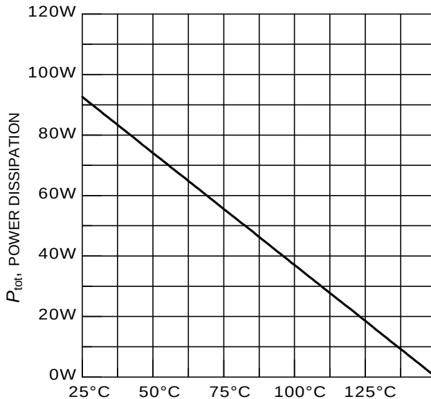
Figure 3. Power dissipation as a function of case temperature ( T_i \leq 150^\circ\text{C} )
