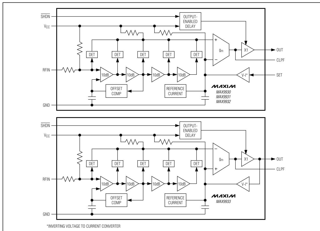
Figure 1. Functional Diagram
