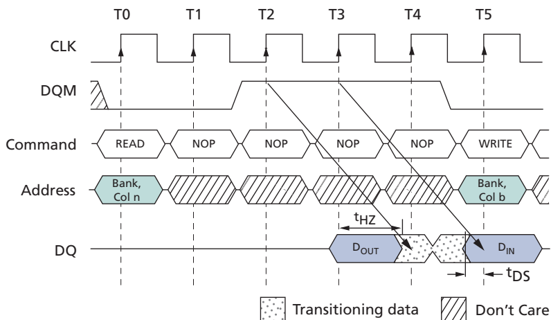
Figure 18: READ-to-WRITE With Extra Clock Cycle
