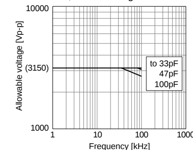
U2J char., Rated Voltage: DC3.15kV
