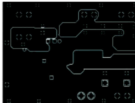
Figure 31. Mid Layer 2
