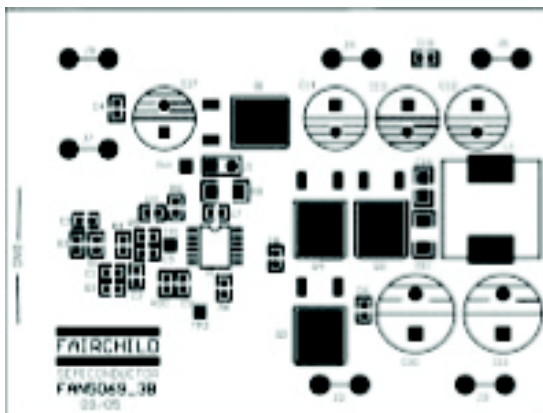
Figure 28. Assembly Diagram
