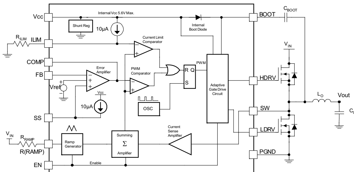
Figure 21. Block Diagram
