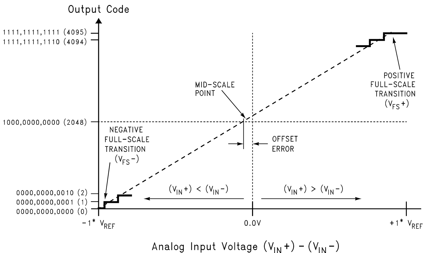
Figure 3. Transfer Characteristic
