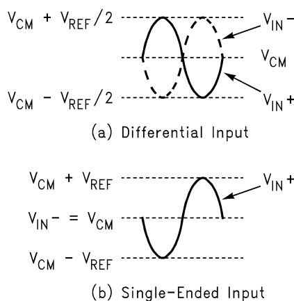
Figure 18. Expected Input Signal Range
