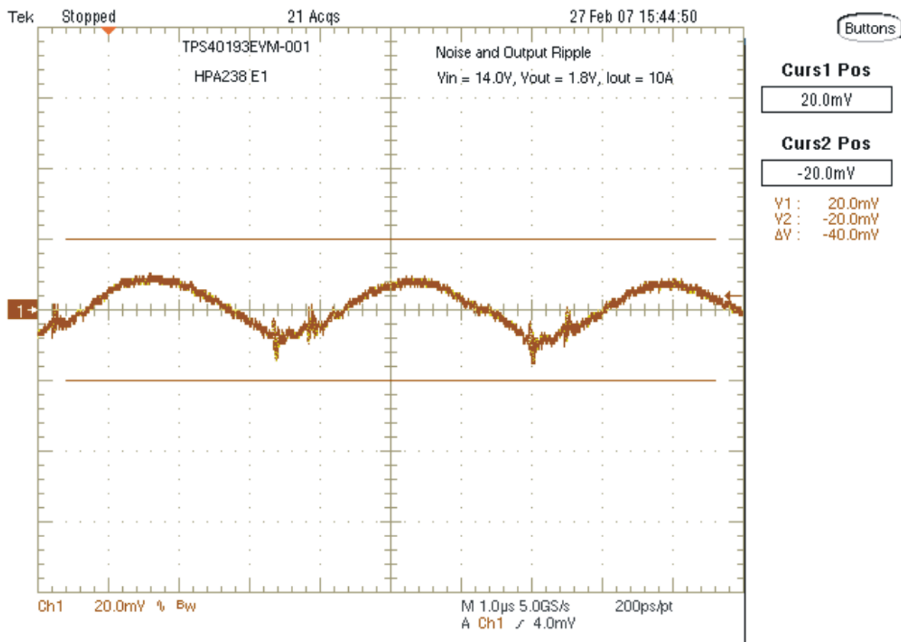
Figure 6-3. TPS40193EVM-001 Output Voltage Ripple
