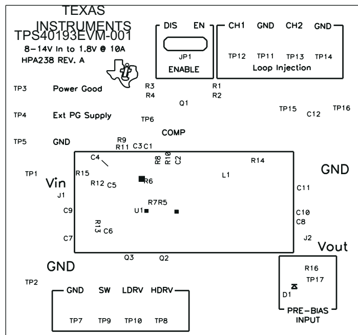
Figure 7-2. TPS40193EVM-001 Silkscreen
