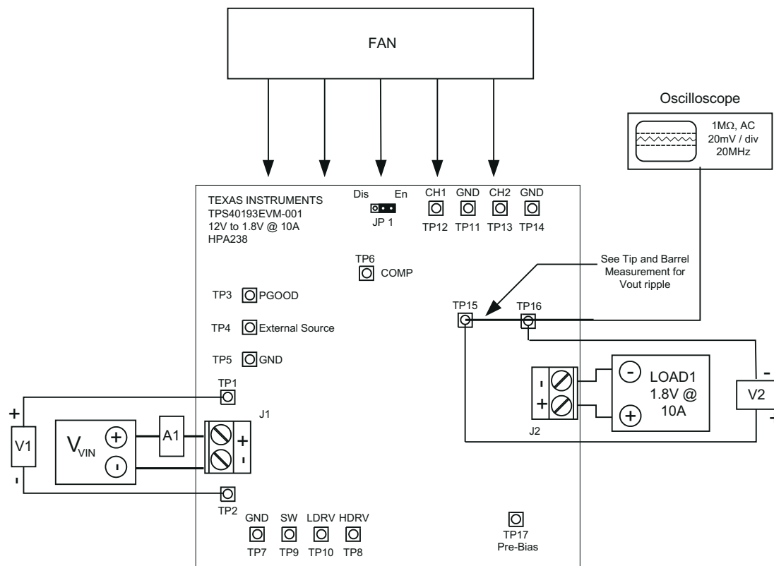
Figure 5-1. TPS40193EVM-001 Recommended Test Setup
