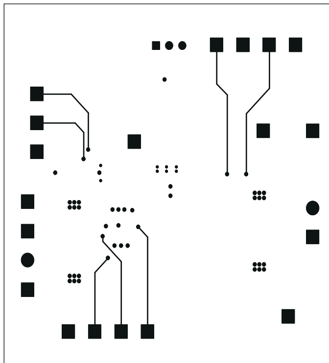
Figure 7-5. TPS40193EVM-001 Internal Layer 1
