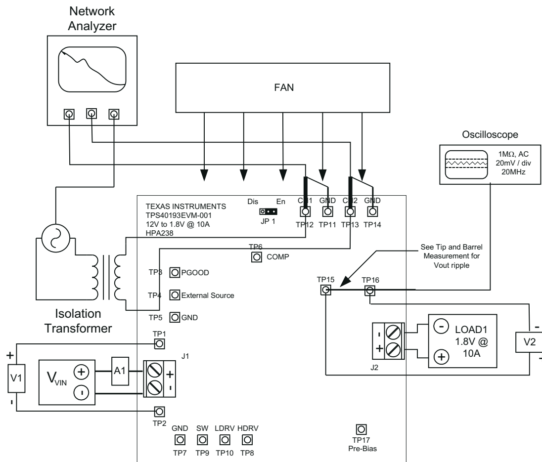
Figure 5-3. TPS40193EVM-001 Control Loop Measurement Setup
