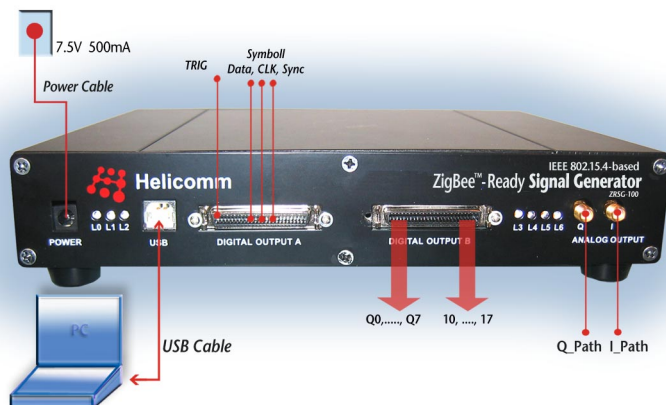
ZRSG-0100 output ports and cable connections
