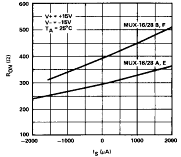
R_{ON} vs SWITCH CURRENT ( I_S )
