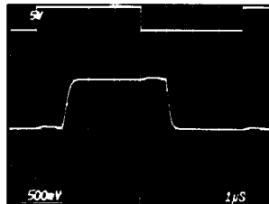
SMALL-SIGNAL SWITCHING WITH FILTERING
