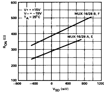
R_{ON} vs SWITCH VOLTAGE ( V_{SD} )
