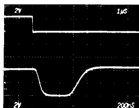
BREAK-BEFORE-MAKE SWITCHING
