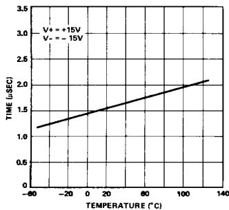
TRANSITION TIME vs TEMPERATURE
