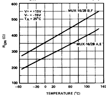
R_{ON} vs TEMPERATURE (T)
