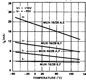
SUPPLY CURRENTS vs TEMPERATURE (T)
