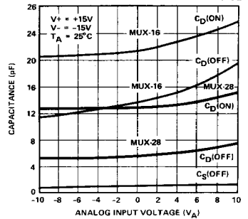
SWITCH CAPACITANCES vs ANALOG INPUT VOLTAGE ( V_A )
