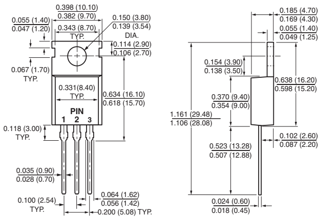
TO-220AB
