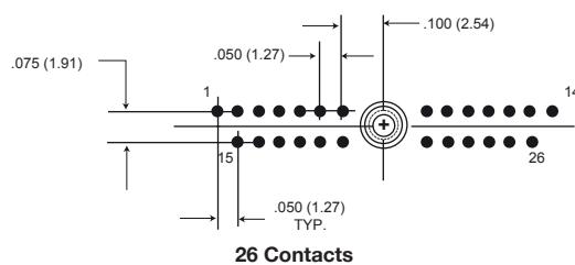
26 Contacts
