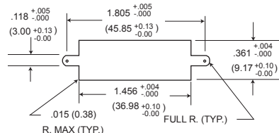
Figure 1 Front Mounting
