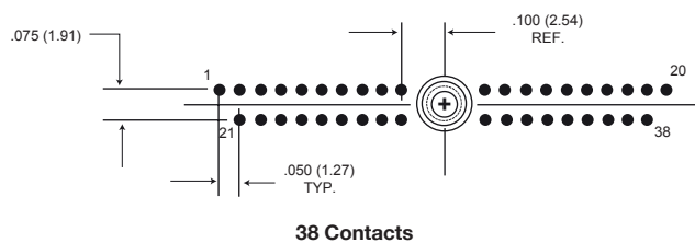
38 Contacts
