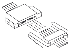
03 End Latches
