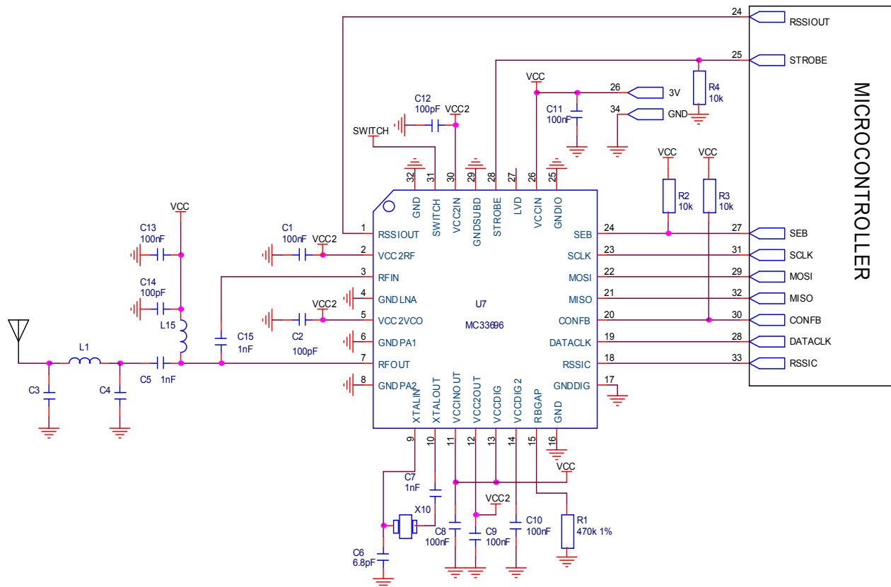
The ON/OFF sequencing for the receiver is controlled by driving a low or high level by the MCU on STROBE pin.
