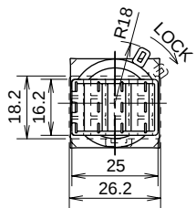
Solder/Tab Terminal
