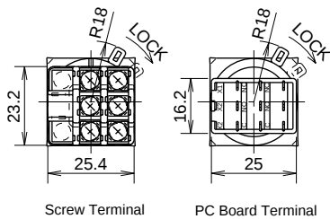
Screw Terminal
