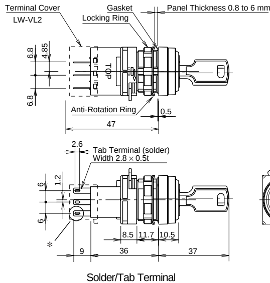
Solder/Tab Terminal
