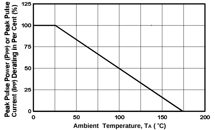
FIGURE 2. PULSE DERATING CURVE
