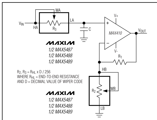
Figure 6. Programmable Filter
