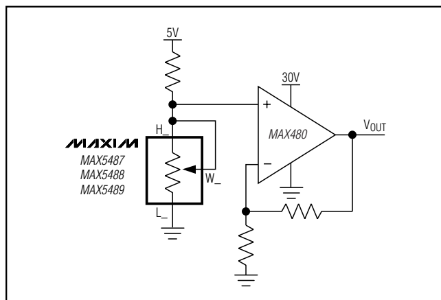
Figure 5. Positive LCD-Bias Control Using a Variable Resistor
