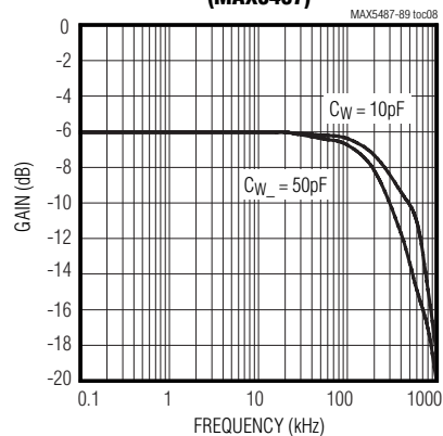
MIDSCALE FREQUENCY RESPONSE (MAX5487)
