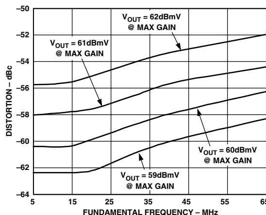
Figure 1. Worst Harmonic Distortion vs. Gain Control
