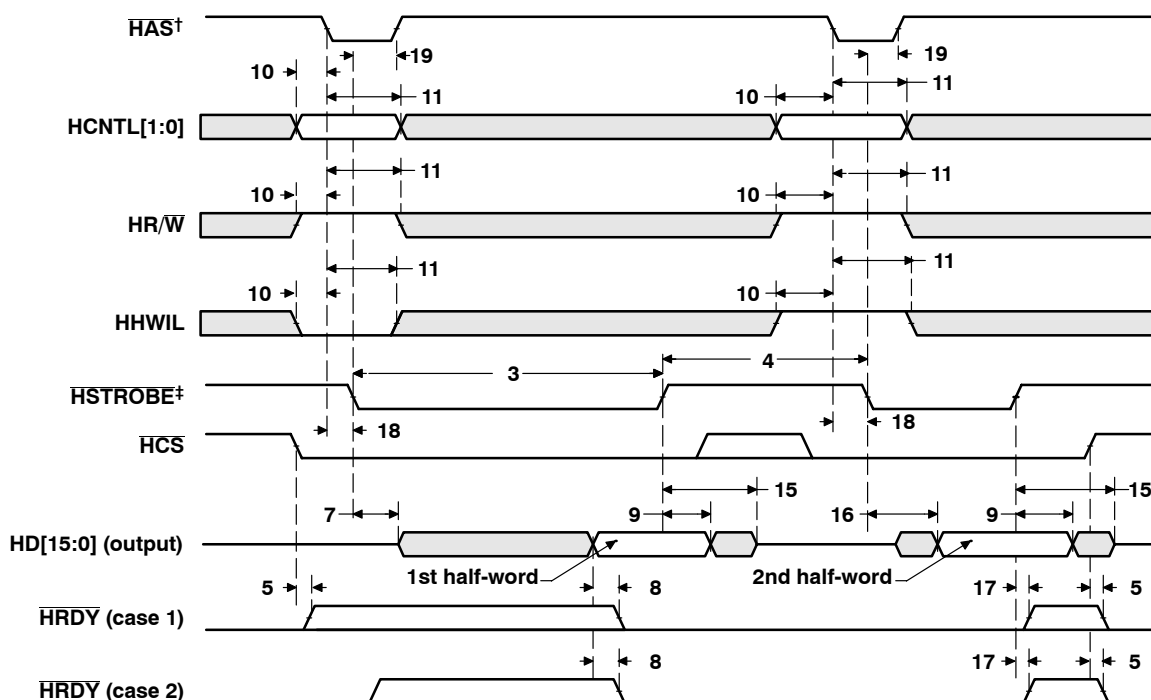
Figure 47. HPI Read Timing ( \overline{HAS} Used)
