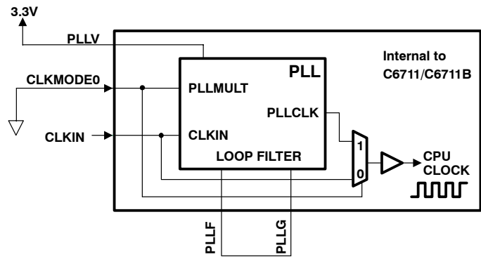
Figure 9. External PLL Circuitry for x1 (Bypass) Mode Only [C6711/11B]
