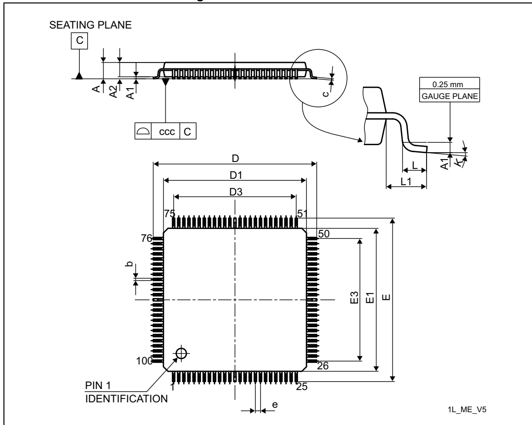
Figure 81. LQFP100 outline
