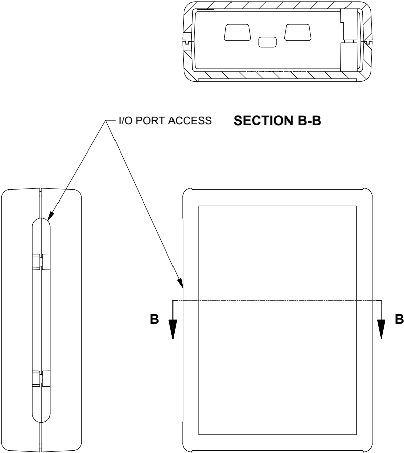
ASSEMBLY - VIEW FROM TOP SIDE
