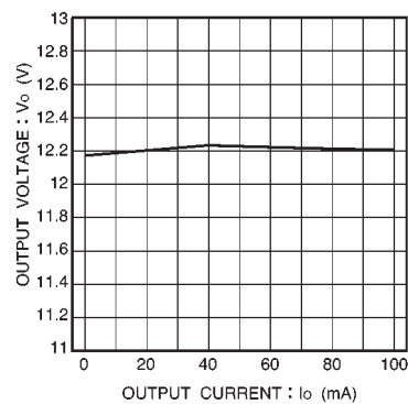
Fig.9 Output characteristic
