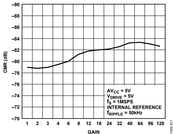
Figure 17. Common-Mode Rejection vs. Gain
