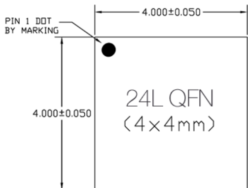
Figure 19. Package Drawing
