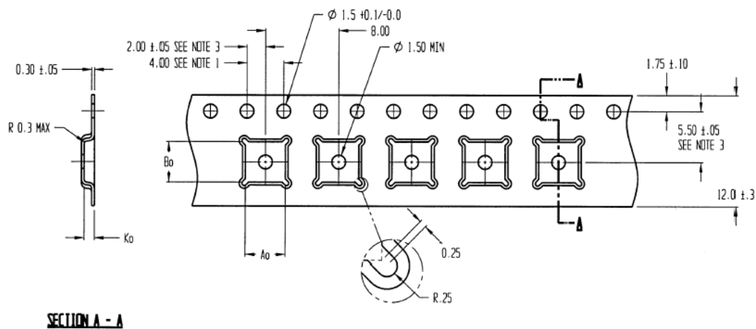
Figure 20. Tape and Reel Drawing
