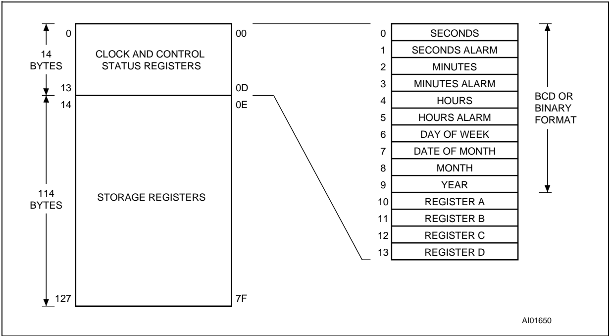
Figure 12. Address Map
