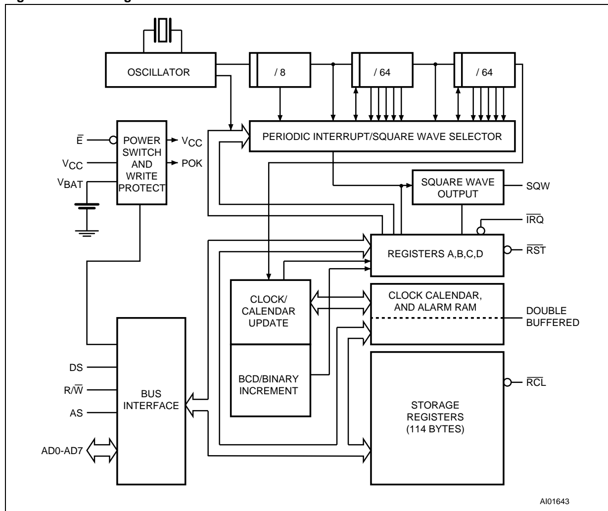
Figure 6. Block Diagram
