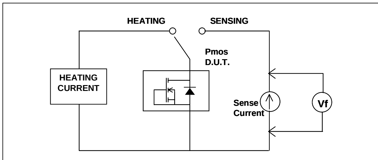
Figure 1: Schematic of temperature measurements
