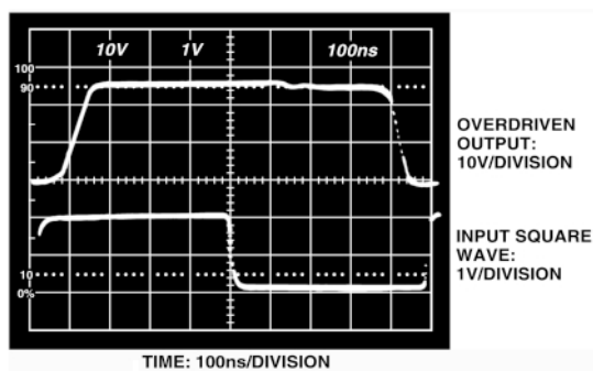
Figure 26. Overdrive Recovery
