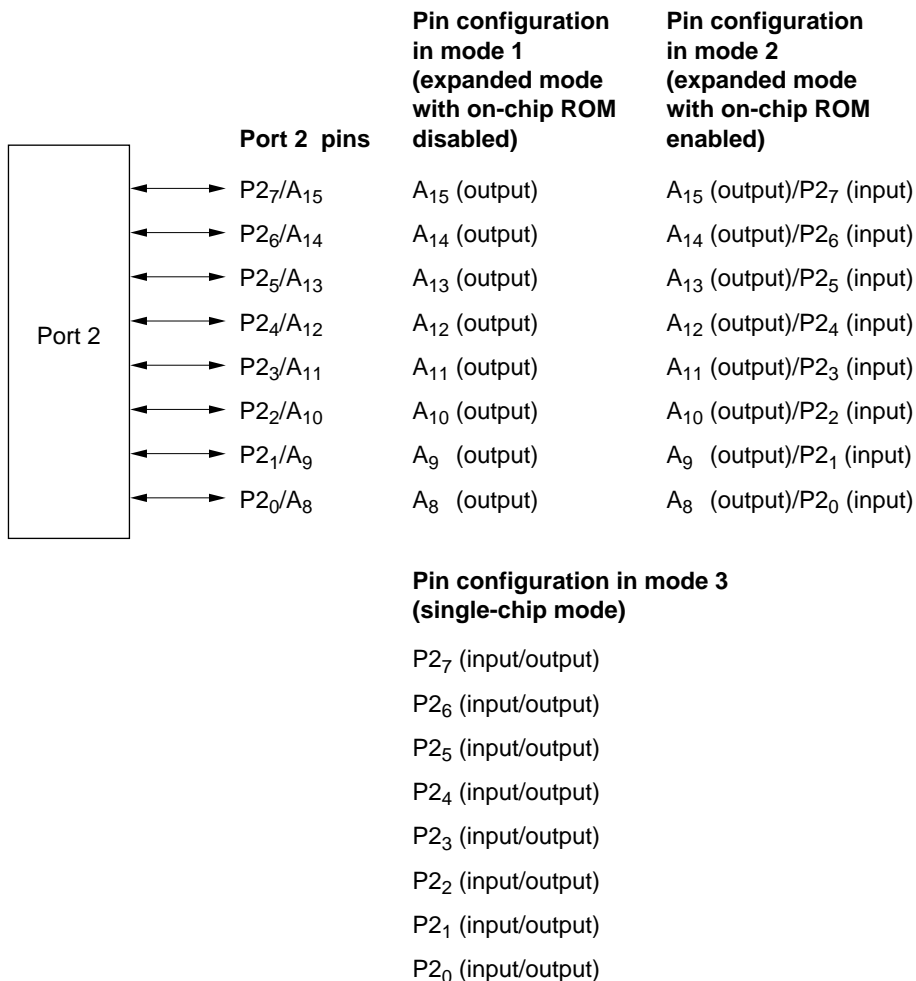
Figure 7-5 Port 2 Pin Configuration
