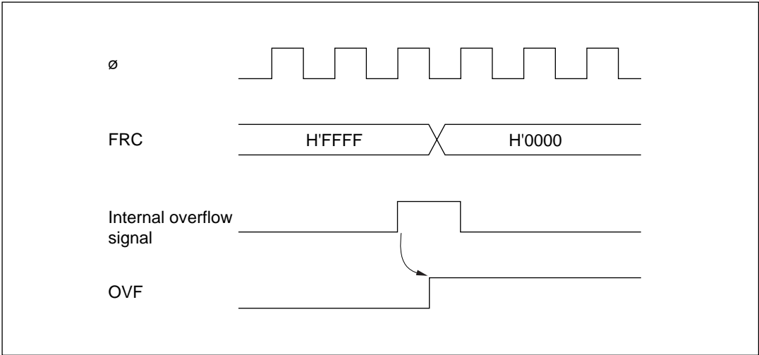
Figure 8-14 Setting of Timer Overflow Flag (OVF)
