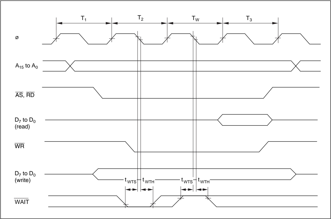
Figure 22-5 Basic Bus Cycle (with 1 Wait State) in Expanded Modes (Modes 1 and 2)
