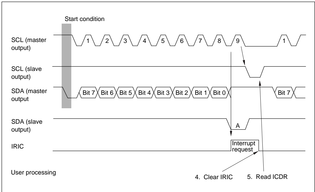
Figure 13-9 Operation Timing in Slave Receive Mode (MLS = WAIT = ACK = ACKB = 0)
