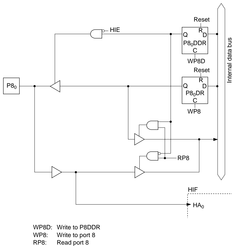
Figure C-8 (a) Port 8 Block Diagram (Pin P8 0 )
