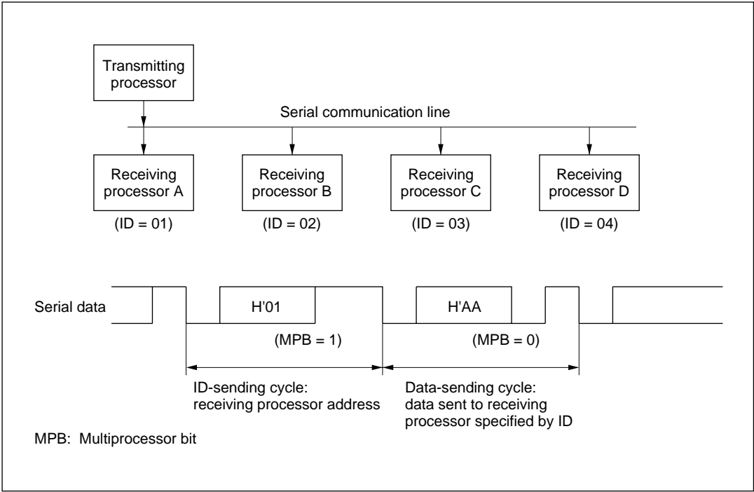
Figure 12-9 Example of Communication among Processors using Multiprocessor Format (Sending Data H'AA to Receiving Processor A)
