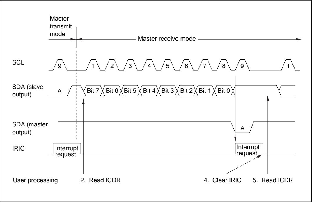
Figure 13-7 Operation Timing in Master Receive Mode (MLS = WAIT = ACK = ACKB = 0)
