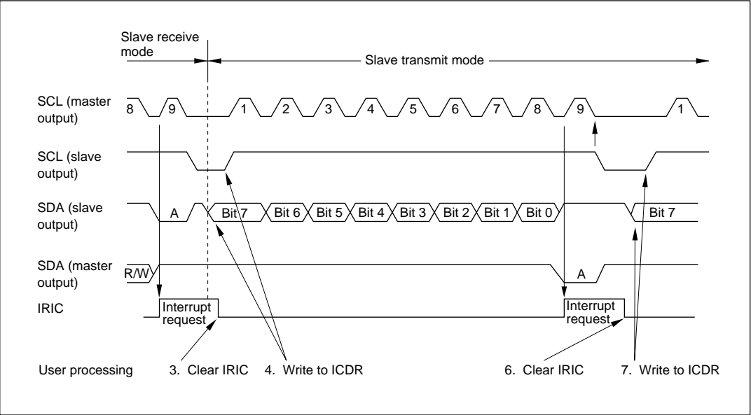
Figure 13-8 Operation Timing in Slave Transmit Mode (MLS = WAIT = ACK = 0)
