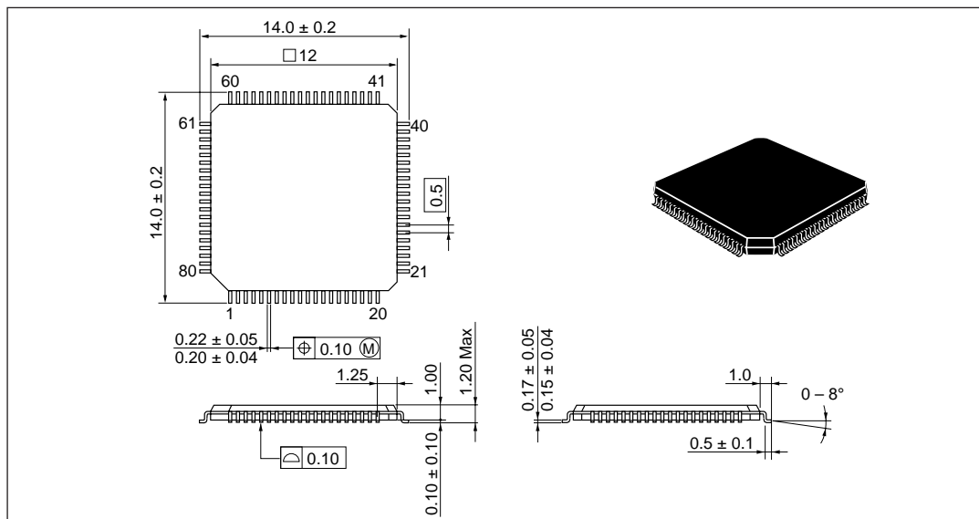
Figure H-2 Package Dimensions (TFP-80C)
