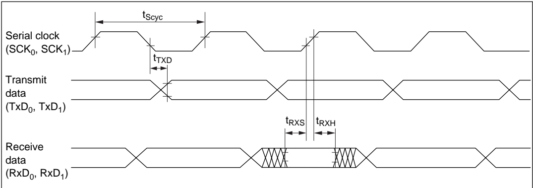
Figure 22-16 SCI Input/Output Timing (Synchronous Mode)
