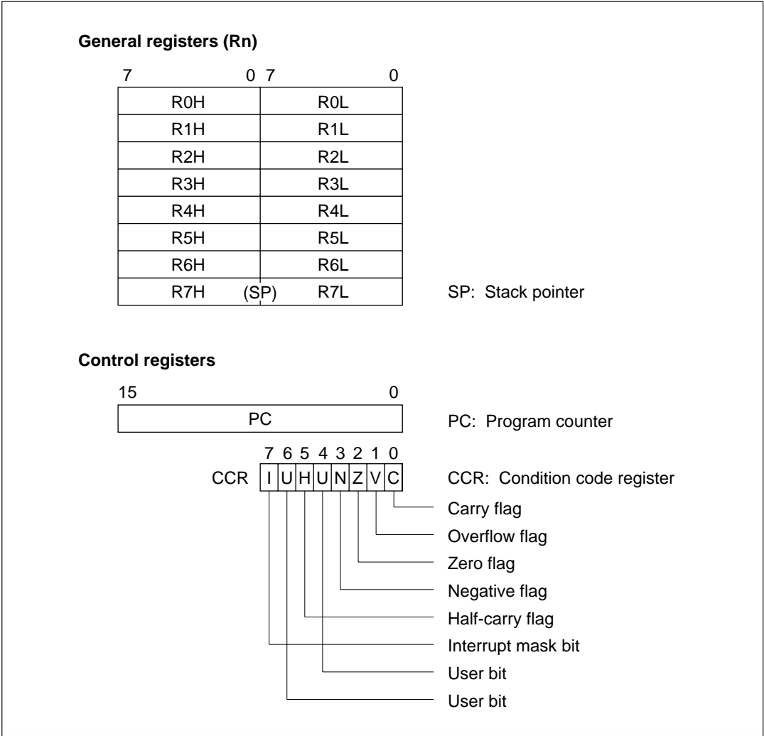
Figure 2-1 CPU Registers
