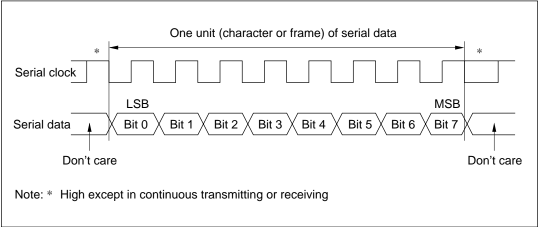
Figure 12-12 Data Format in Synchronous Communication
