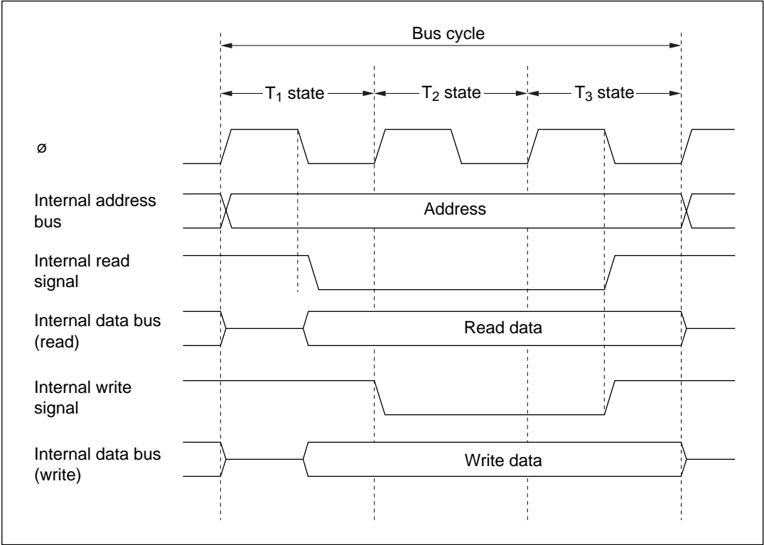
Figure 2-15 On-Chip Supporting Module Access Cycle
