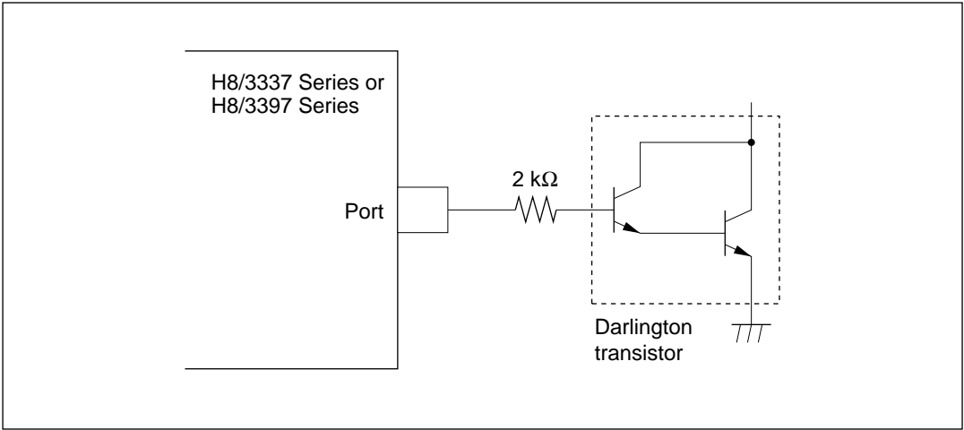
Figure 22-1 Example of Circuit for Driving a Darlington Transistor (5-V Version)
