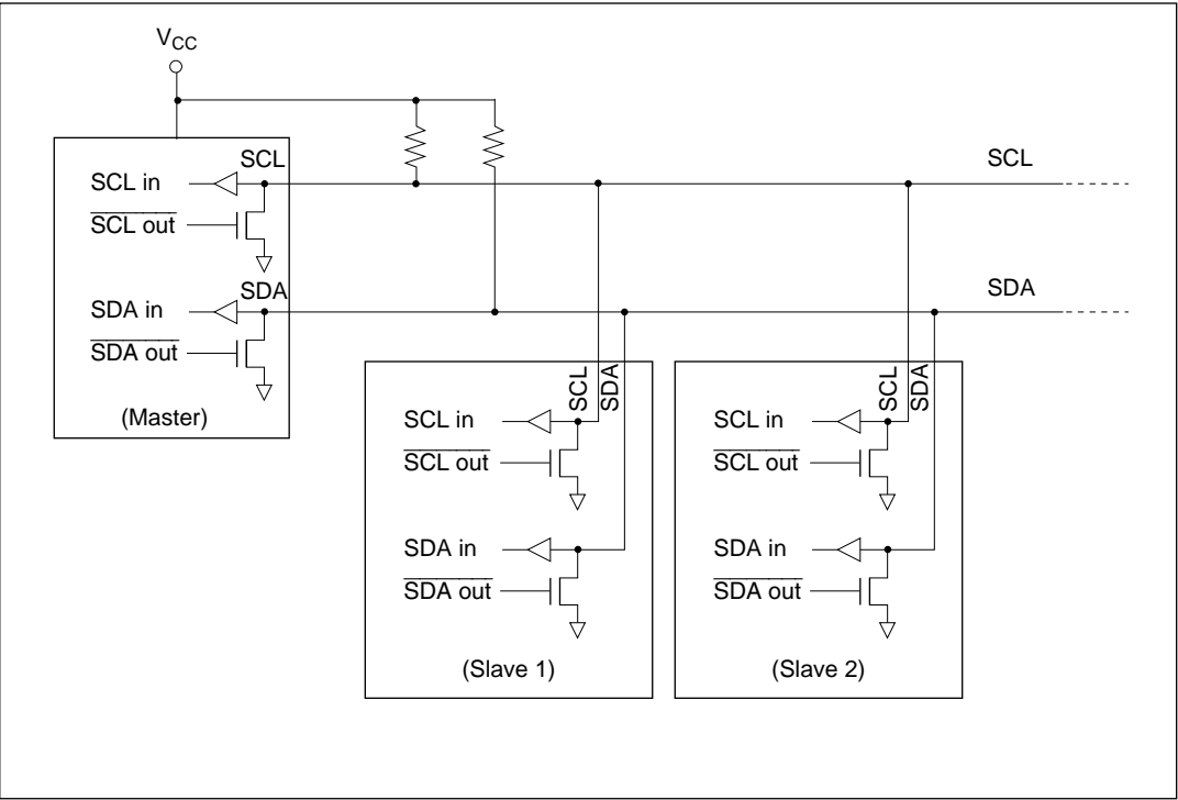
Figure 13-1 I 2 C Bus Interface Connections (Example) (H8/3337 Series Chip as Master)
