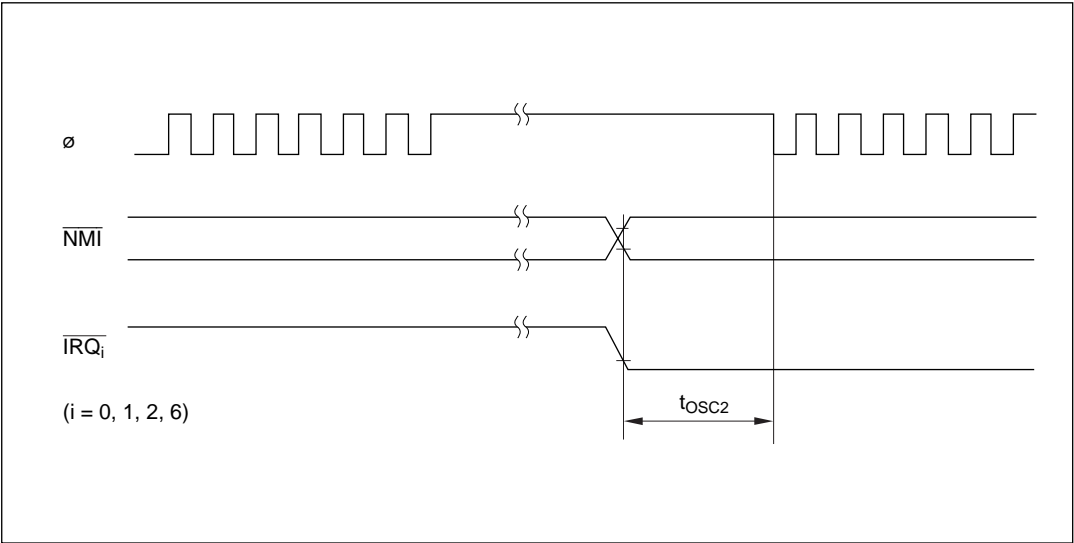
Figure 22-9 Clock Settling Timing for Recovery from Software Standby Mode
