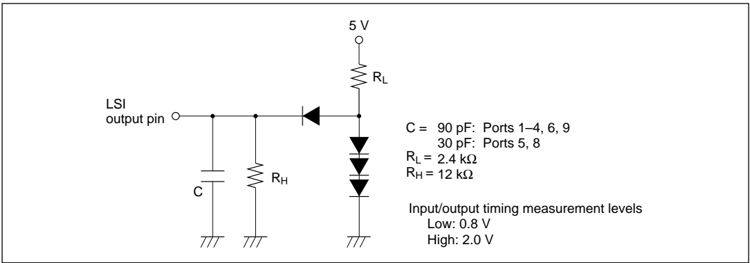
Figure 22-3 Output Load Circuit
