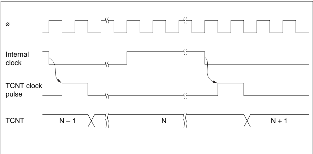
Figure 9-2 Increment Timing for Internal Clock Input
