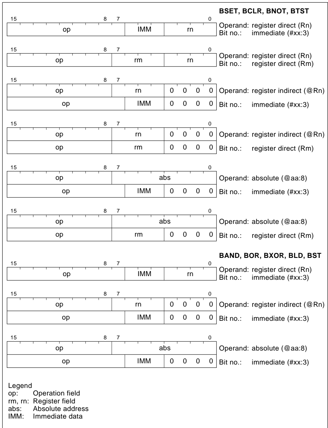
Figure 2-7 Bit Manipulation Instruction Codes (1)
