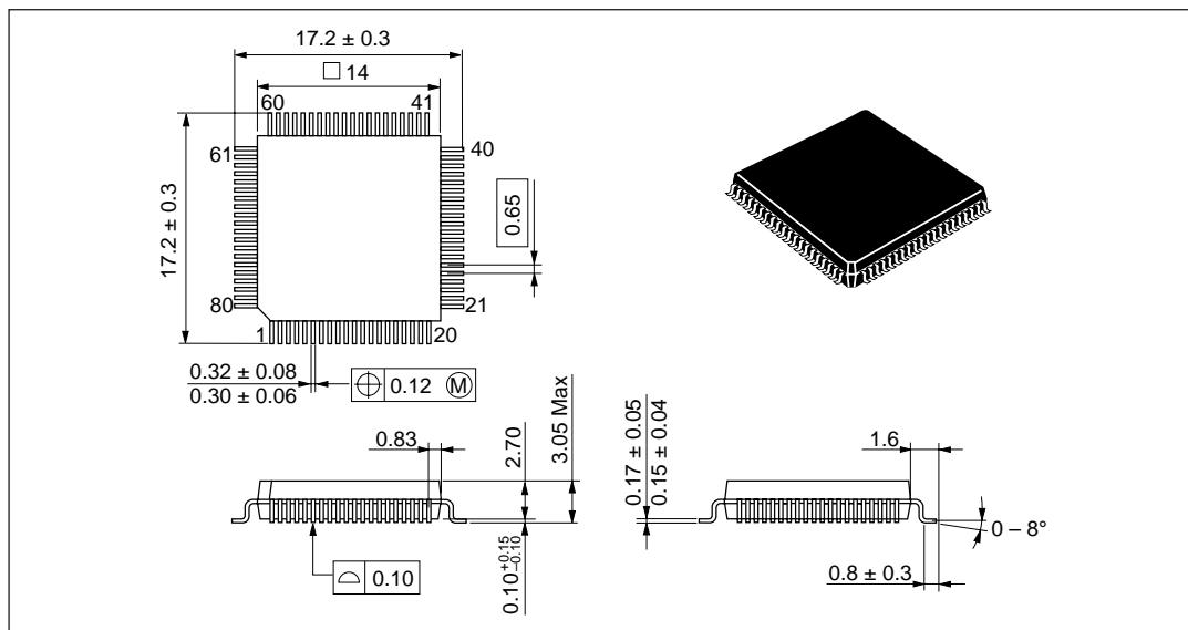
Figure H-1 Package Dimensions (FP-80A)
