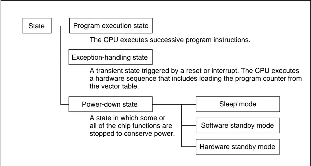
Figure 2-11 Operating States
