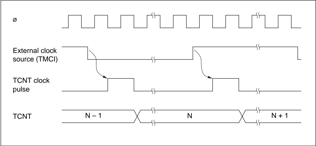
Figure 9-3 Increment Timing for External Clock Input
