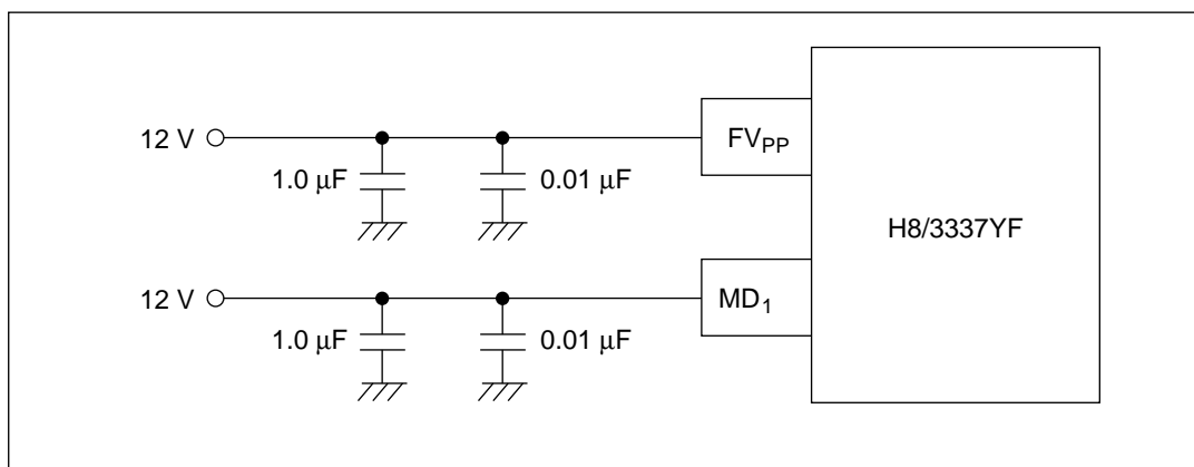
Figure 20-21 V PP Power Supply Circuit Design (Example)
