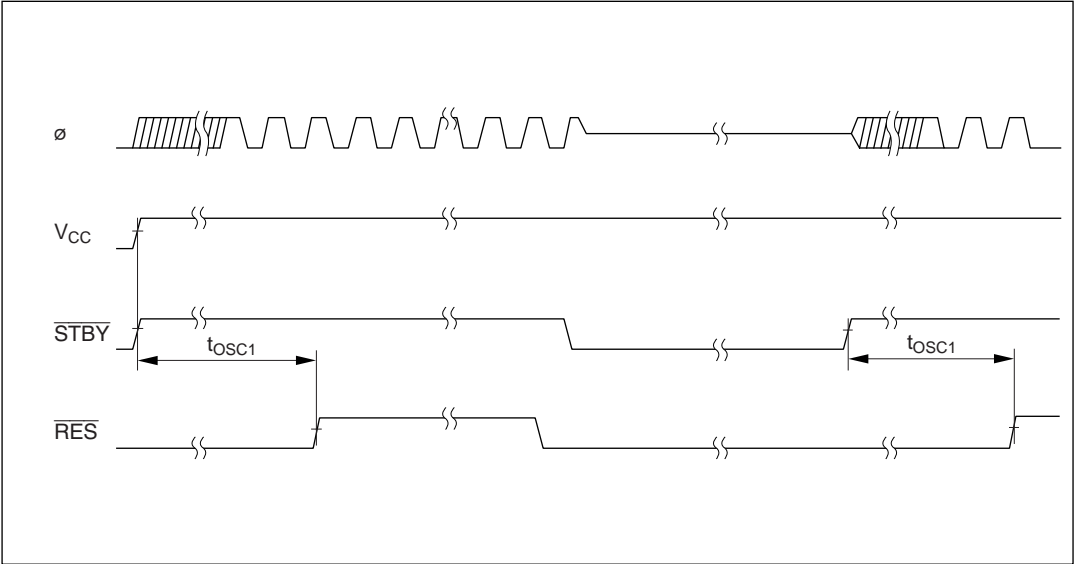
Figure 22-8 Clock Settling Timing
