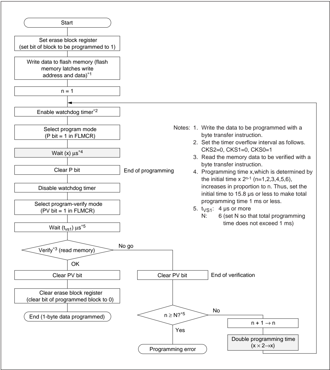
Figure 20-8 Programming Flowchart
