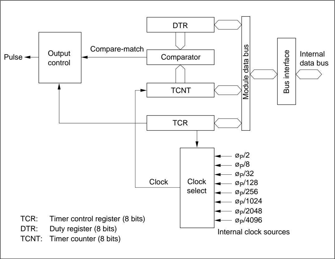
Figure 10-1 Block Diagram of PWM Timer (One Channel)
