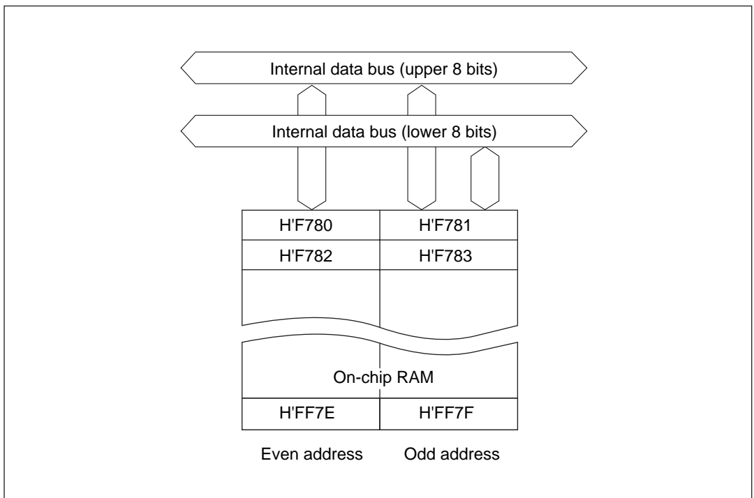
Figure 17-1 Block Diagram of On-Chip RAM (H8/3337Y)
