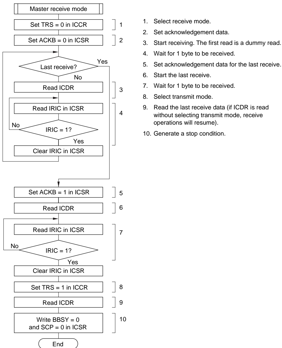
Figure 13-13 Flowchart for Master Receive Mode (Example)
