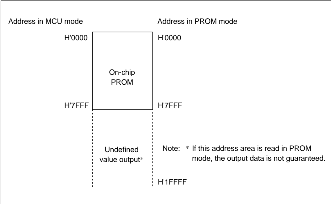
Figure 18-4 H8/3334Y Memory Map in PROM Mode
