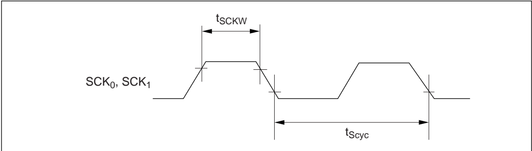
Figure 22-17 SCI Input Clock Timing
