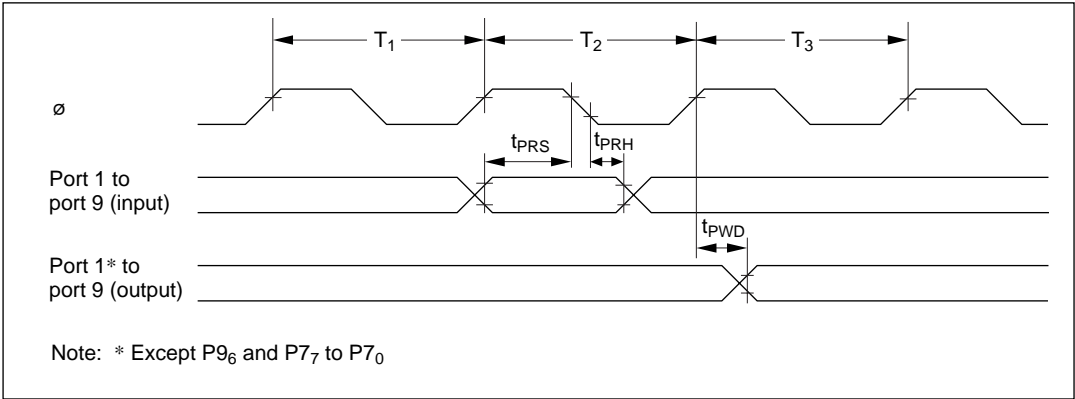
Figure 22-18 I/O Port Input/Output Timing
