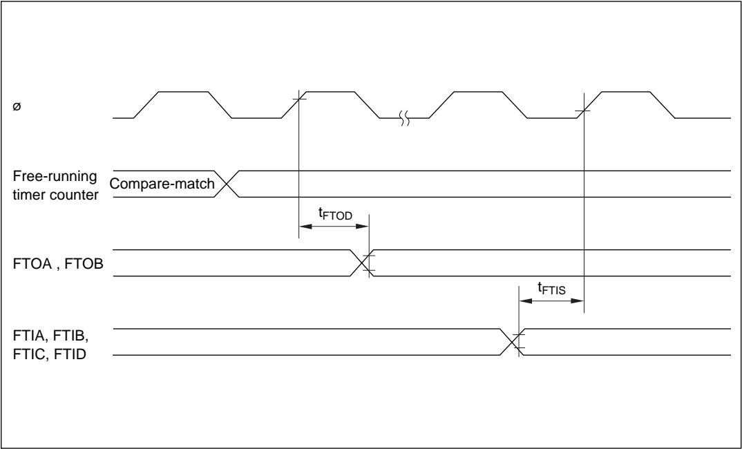
Figure 22-10 Free-Running Timer Input/Output Timing
