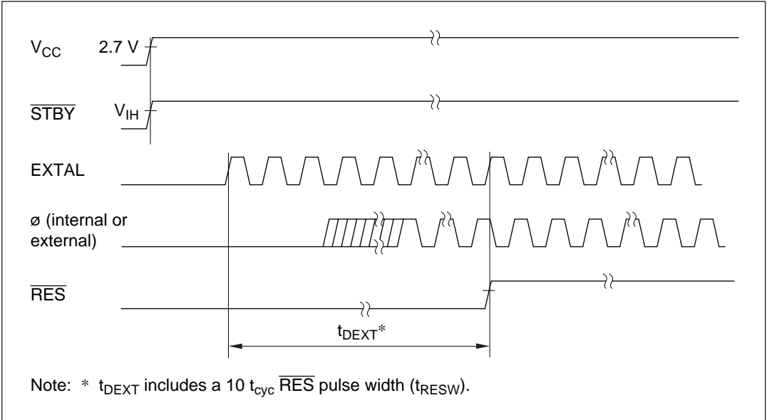
Figure 6-7 External Clock Output Settling Delay Time
