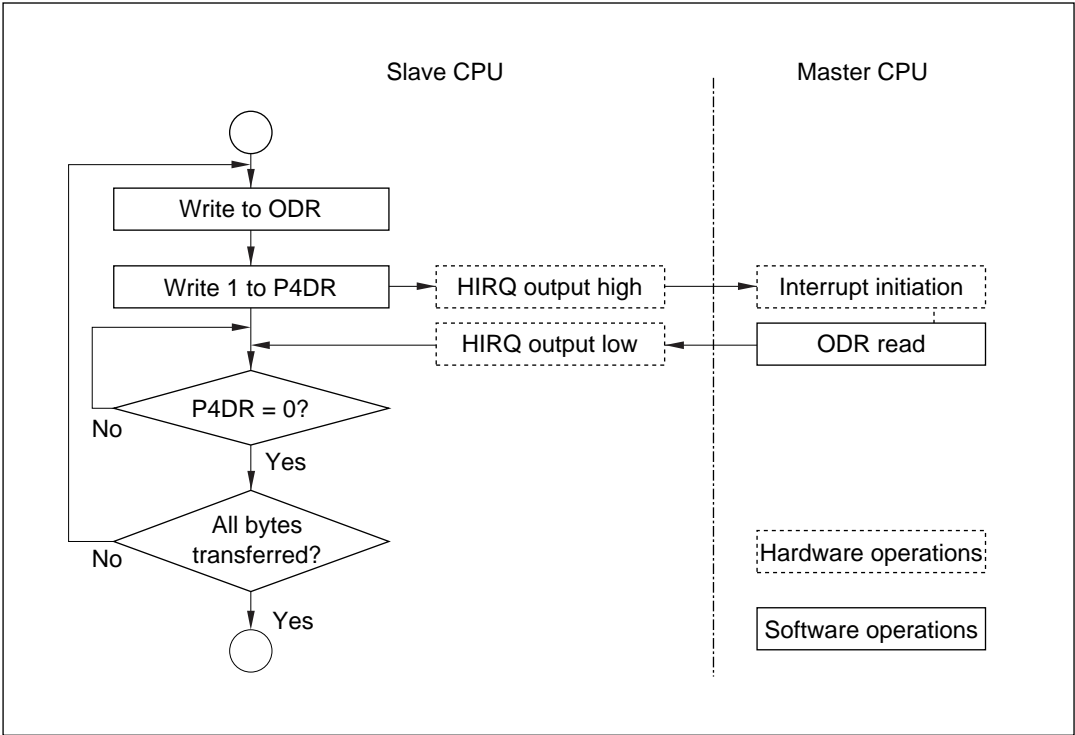
Figure 14-3 HIRQ Output Flowchart
