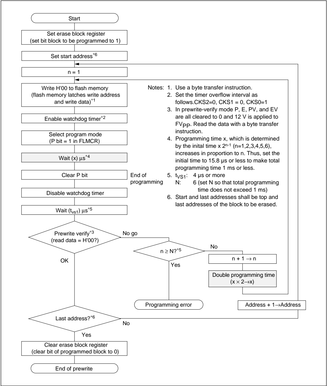
Figure 20-10 Prewrite Flowchart
