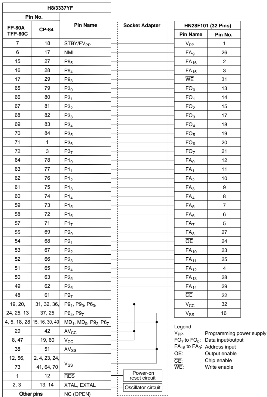
Figure 20-14 Wiring of Socket Adapter
