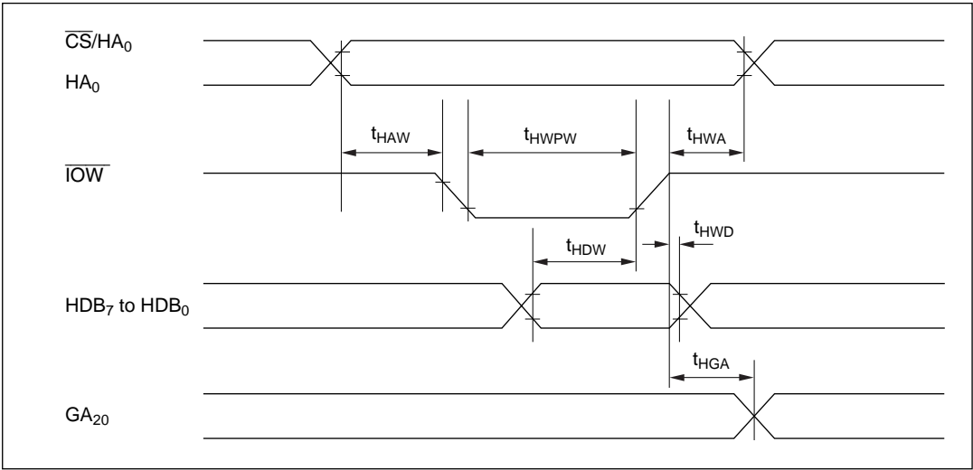
Figure 22-20 Host Interface Write Timing
