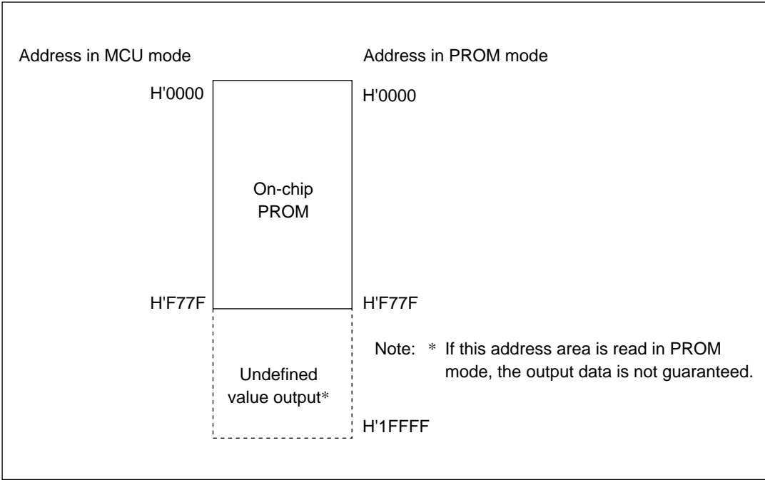
Figure 18-3 H8/3337Y Memory Map in PROM Mode
