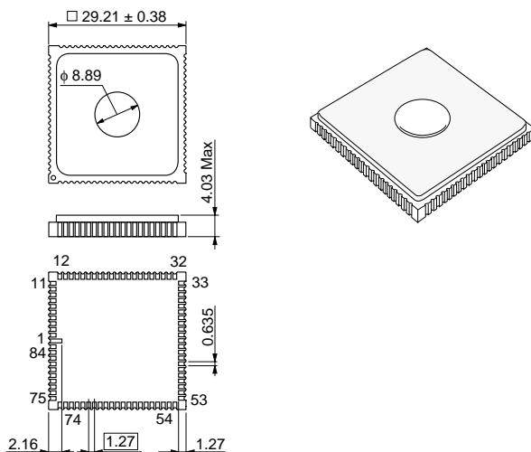
Figure H-4 Package Dimensions (CG-84)
