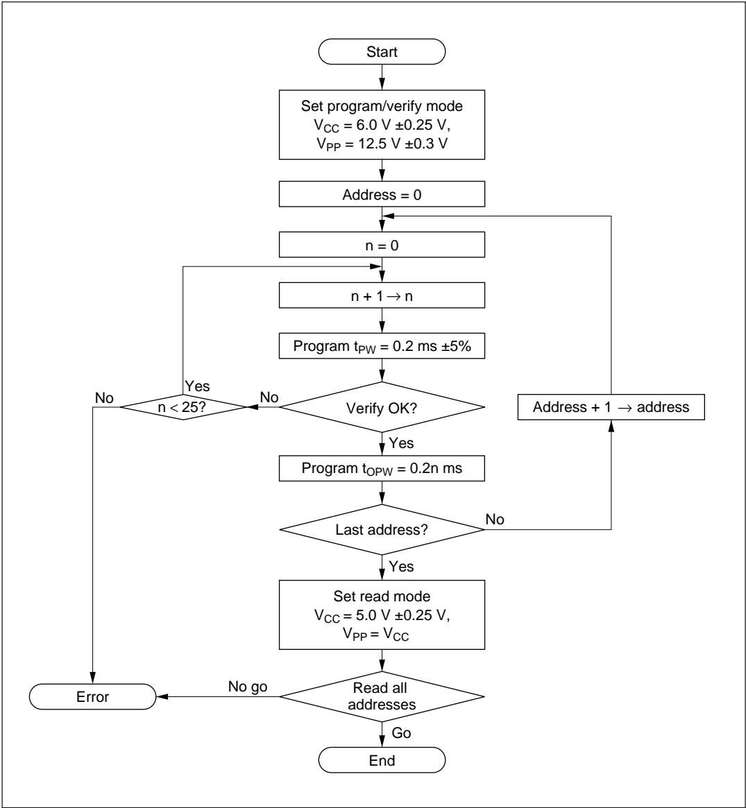
Figure 18-5 High-Speed Programming Flowchart
