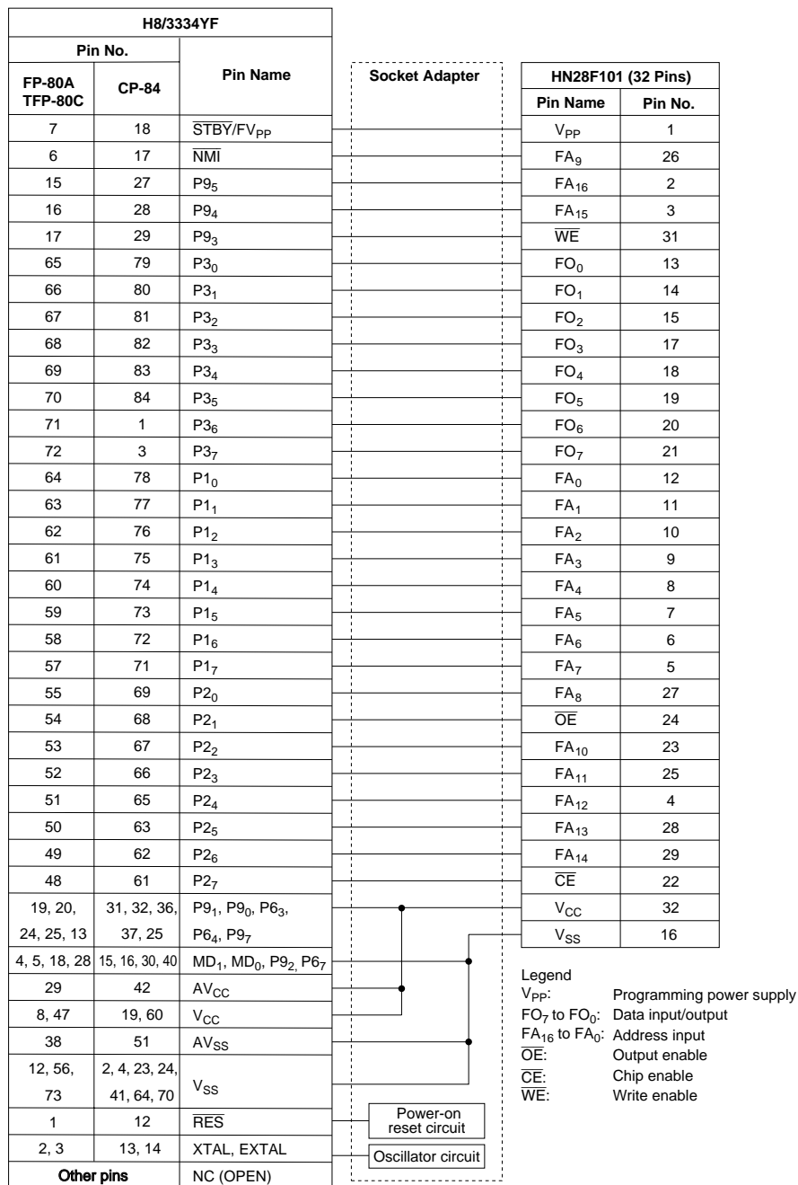
Figure 19-14 Wiring of Socket Adapter
