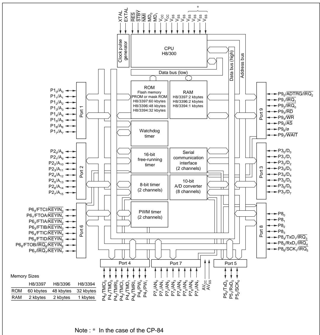
Figure 1-1 (b) Block Diagram for H8/3397 Series
