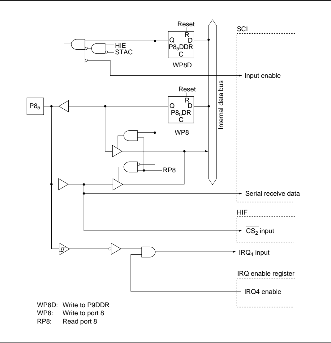
Figure C-8 (e) Port 8 Block Diagram (Pin P8 5 )
