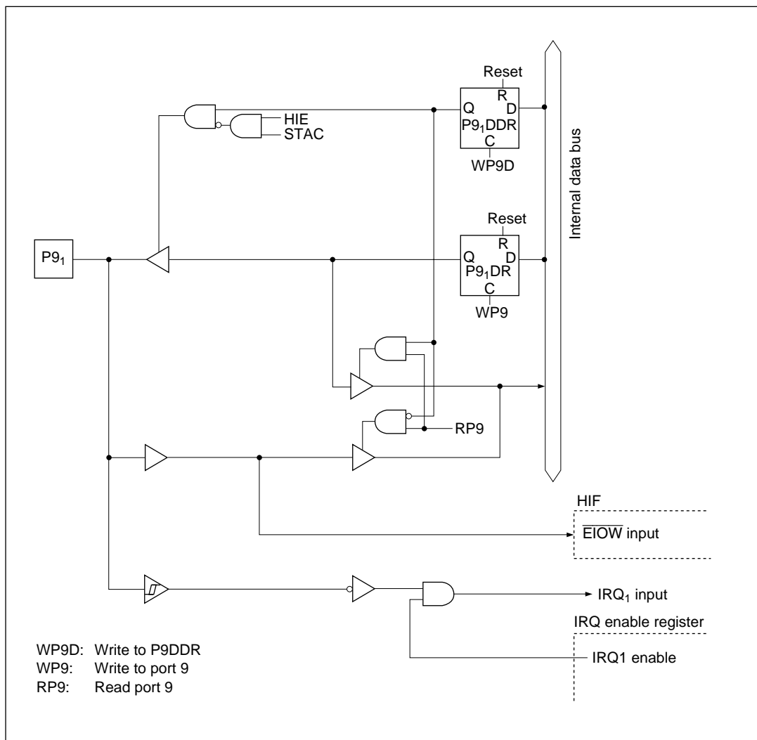
Figure C-9 (b) Port 9 Block Diagram (Pin P9_1 )
