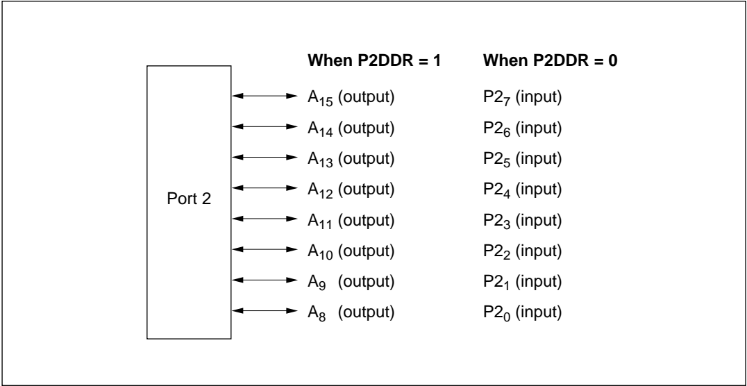
Figure 7-7 Pin Functions in Mode 2 (Port 2)
