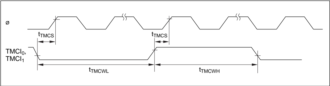
Figure 22-13 8-Bit Timer Clock Input Timing
