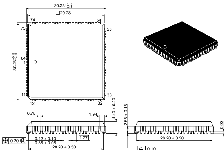
Figure H-3 Package Dimensions (CP-84)
