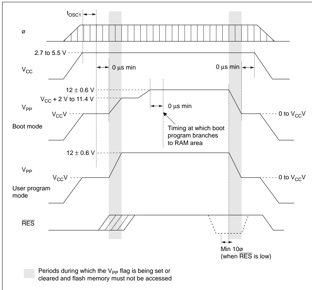
Figure 20-20 V_{\text{pp}} Power-On and Power-Off Timing
