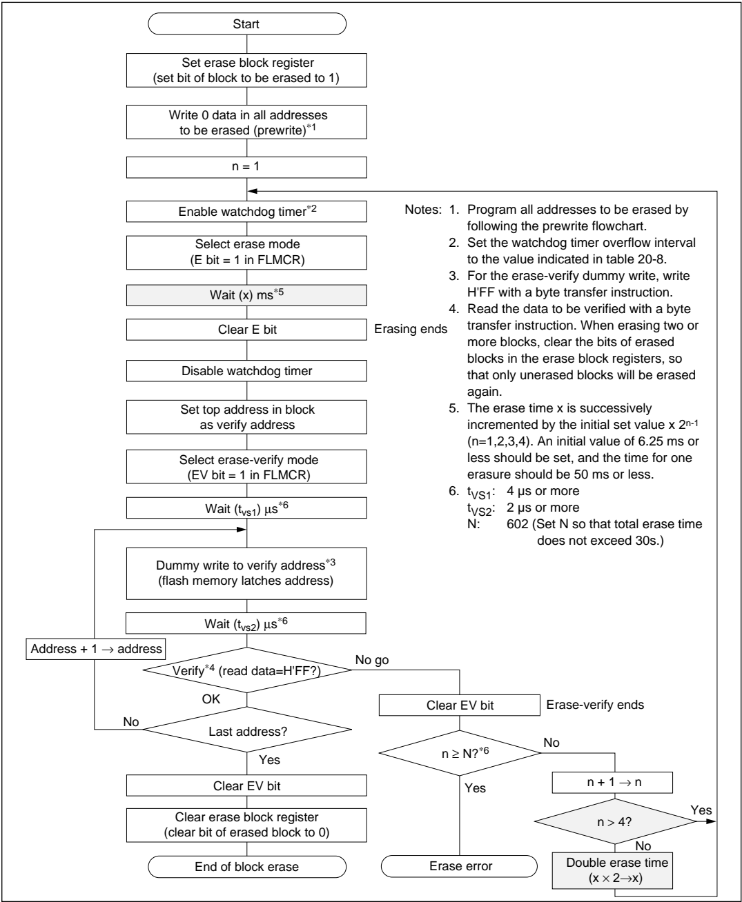
Figure 20-9 Erasing Flowchart
