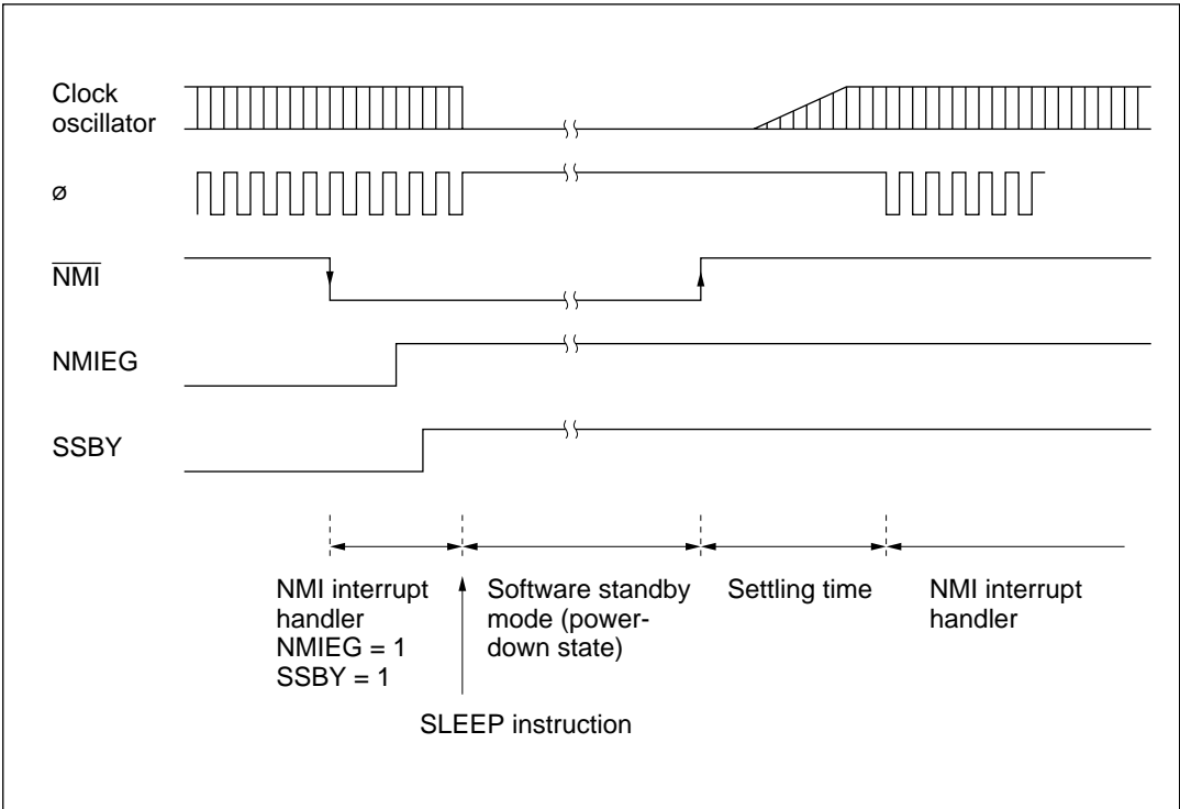
Figure 21-1 NMI Timing in Software Standby Mode (Application Example)
