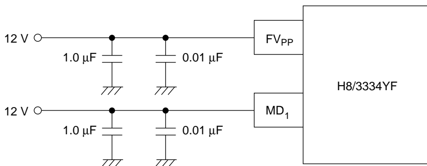
Figure 19-21 V PP Power Supply Circuit Design (Example)
