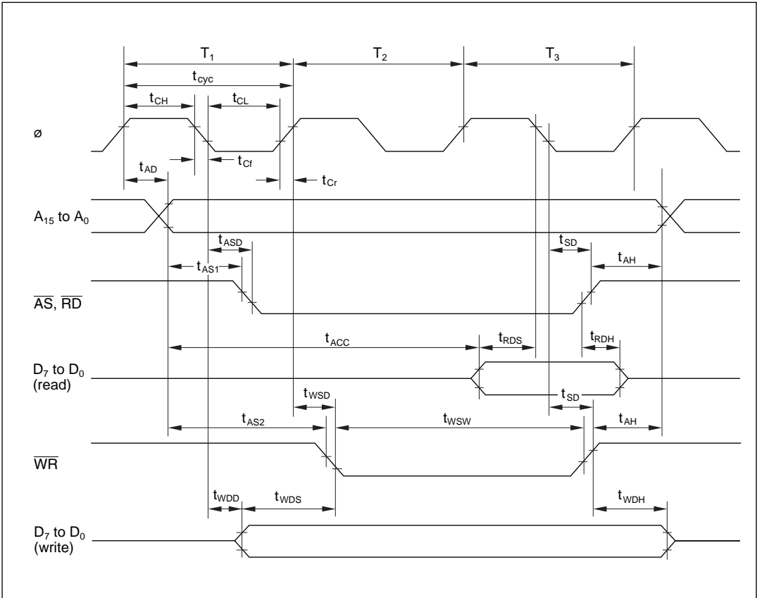
Figure 22-4 Basic Bus Cycle (without Wait States) in Expanded Modes
