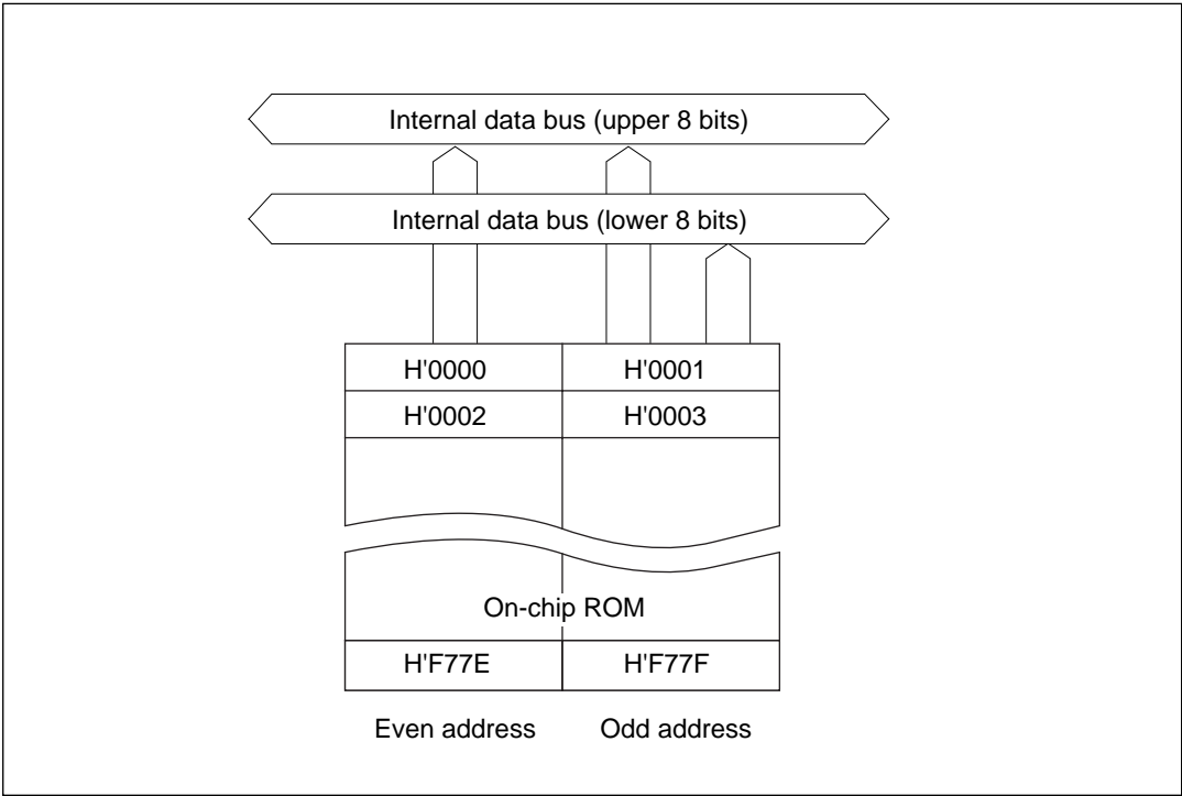
Figure 18-1 Block Diagram of On-Chip ROM (H8/3337Y Single-Chip Mode)
