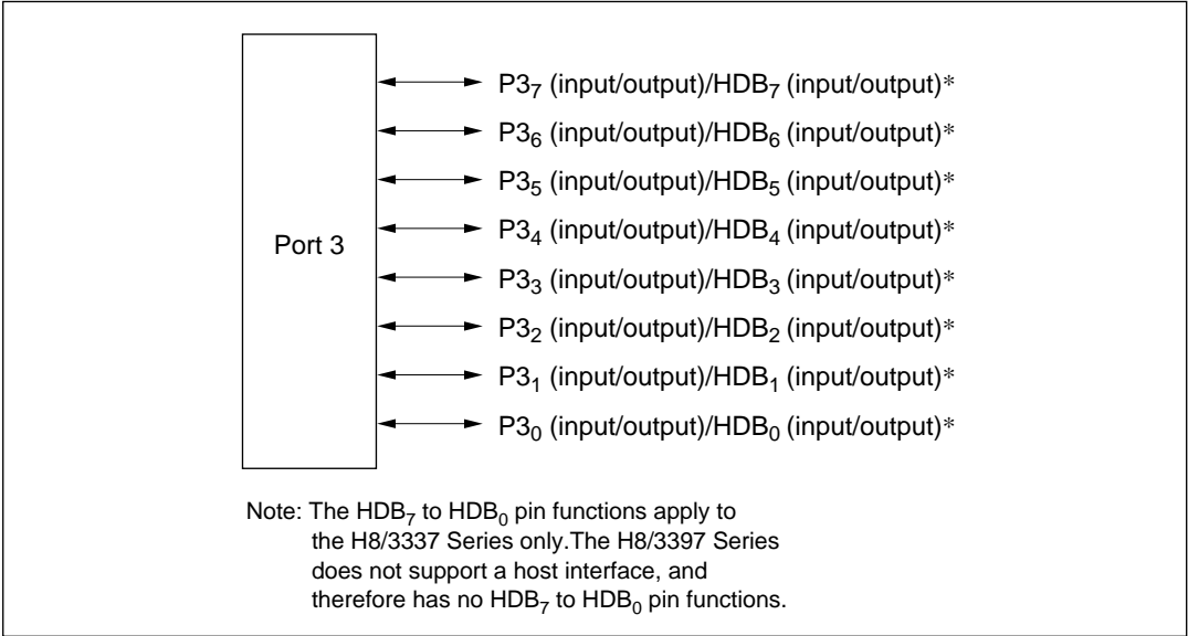
Figure 7-11 Pin Functions in Mode 3 (Port 3)
