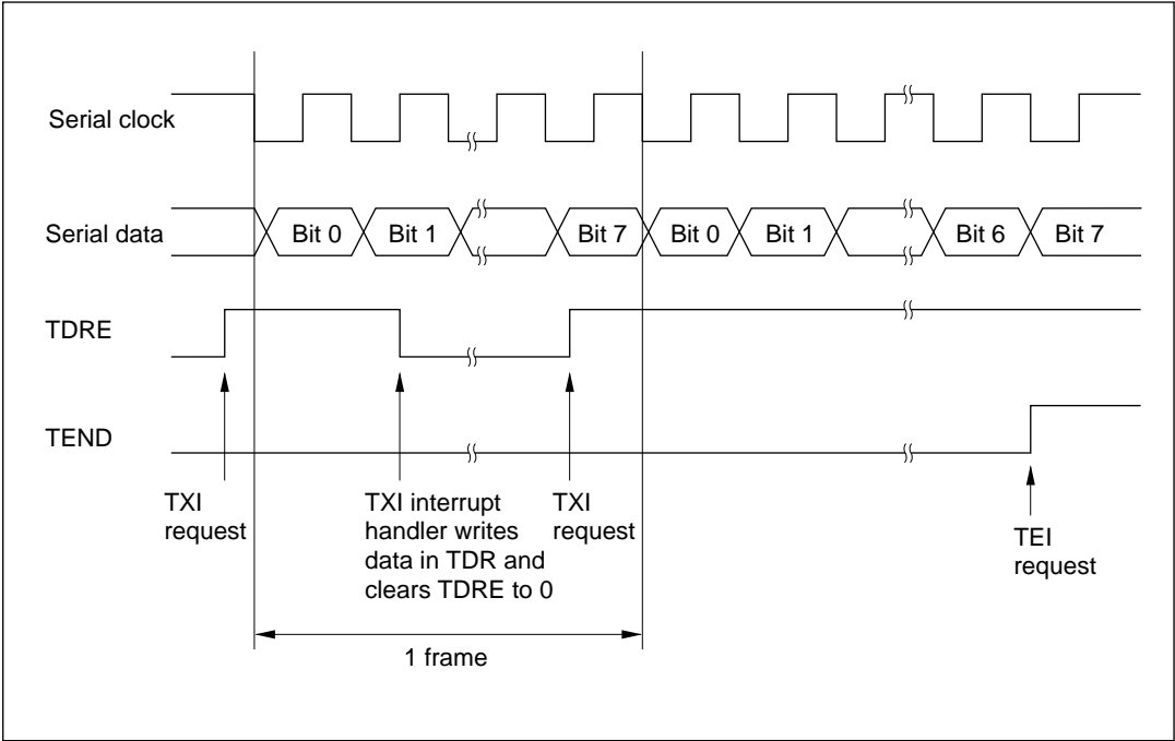
Figure 12-14 Example of SCI Transmit Operation
