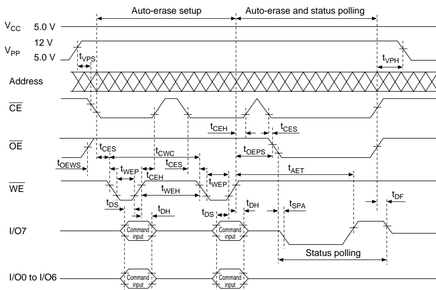
Figure 19-17 Auto-Erase Timing
