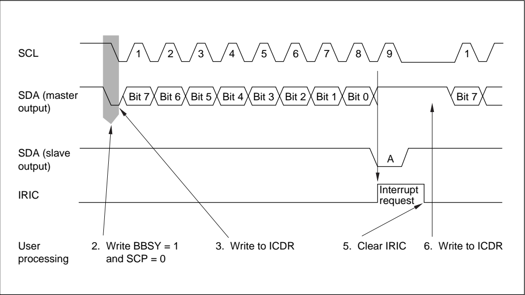
Figure 13-6 Operation Timing in Master Transmit Mode (MLS = WAIT = ACK = 0)
