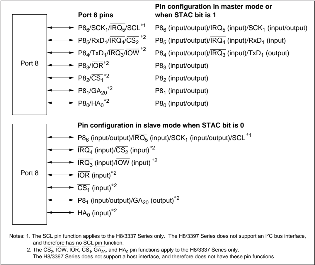
Figure 7-16 Port 8 Pin Configuration
