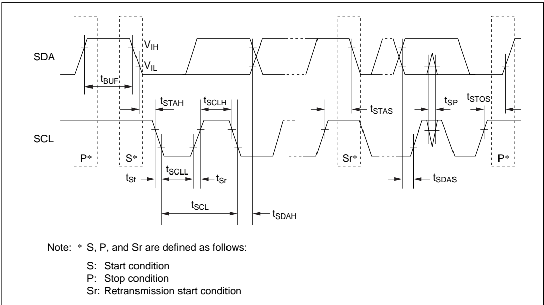
Figure 22-21 I 2 C Interface Input/Output Timing
