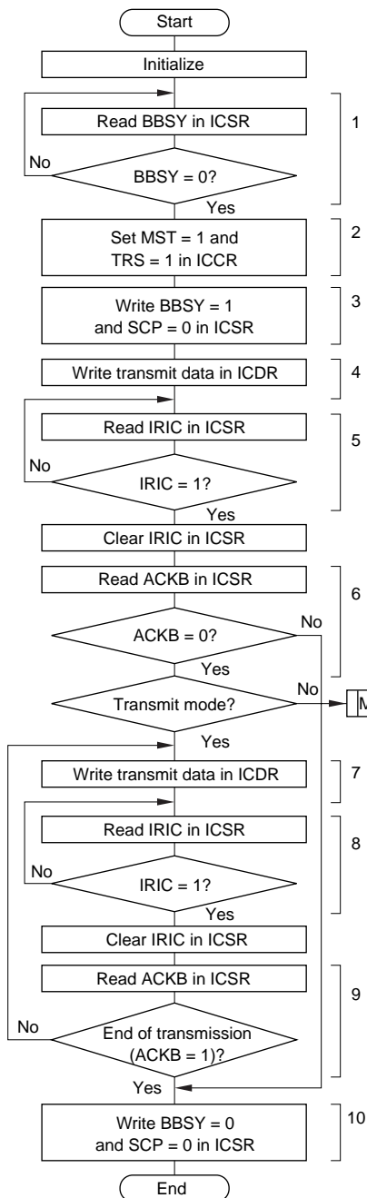
Figure 13-12 Flowchart for Master Transmit Mode (Example)
