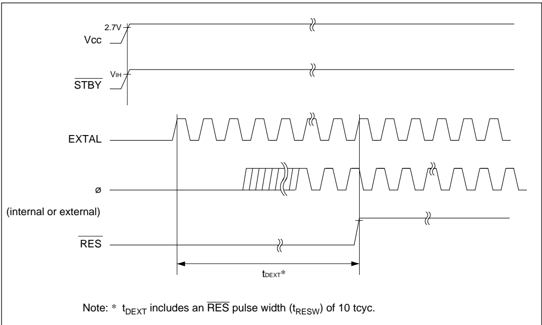
Figure 22-22 External clock output delay Timing
