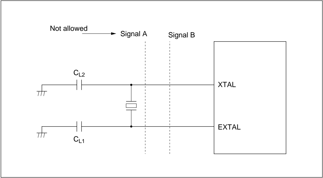
Figure 6-4 Board Design around External Crystal
