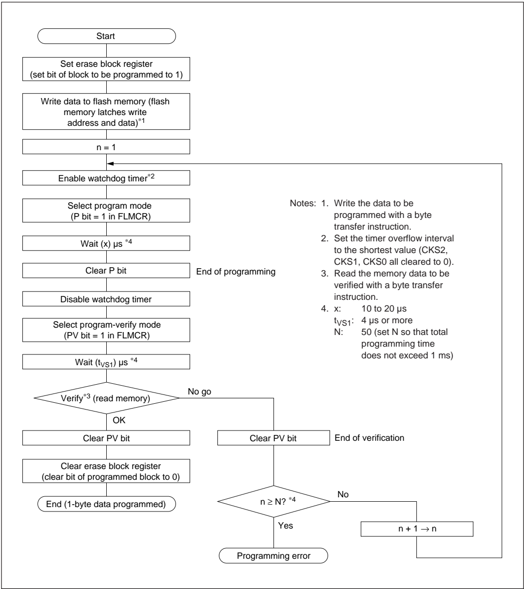
Figure 19-8 Programming Flowchart
