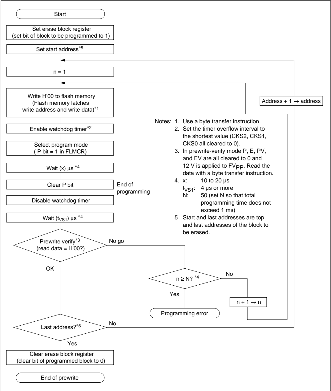
Figure 19-10 Prewrite Flowchart
