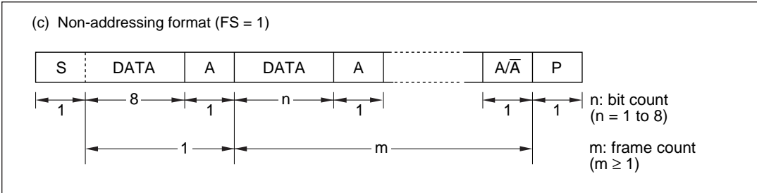
Figure 13-4 I 2 C Bus Data Format (Non-Acknowledge Format)
