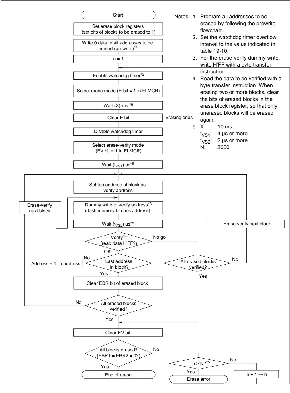
Figure 19-11 Multiple-Block Erase Flowchart
