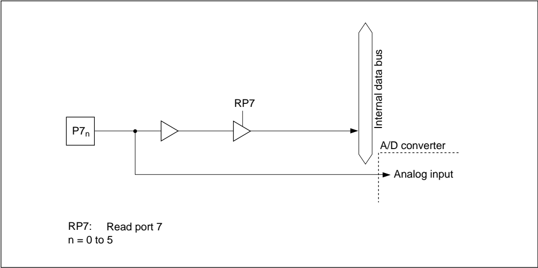
Figure C-7 (a) Port 7 Block Diagram (Pins P7 0 to P7 5 )
