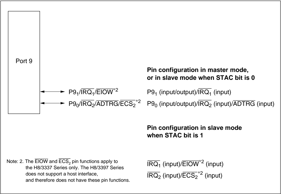
Figure 7-17 Port 9 Pin Configuration (cont)
