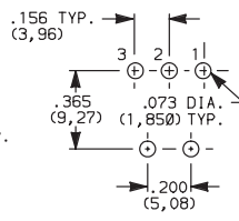
7101MD9A4BE Horizontal Actuation SPDT
