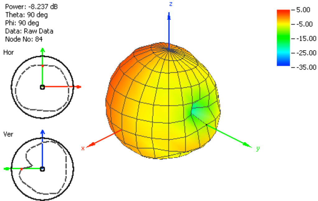
Figure 21. Radiation Pattern at 2460 MHz.
