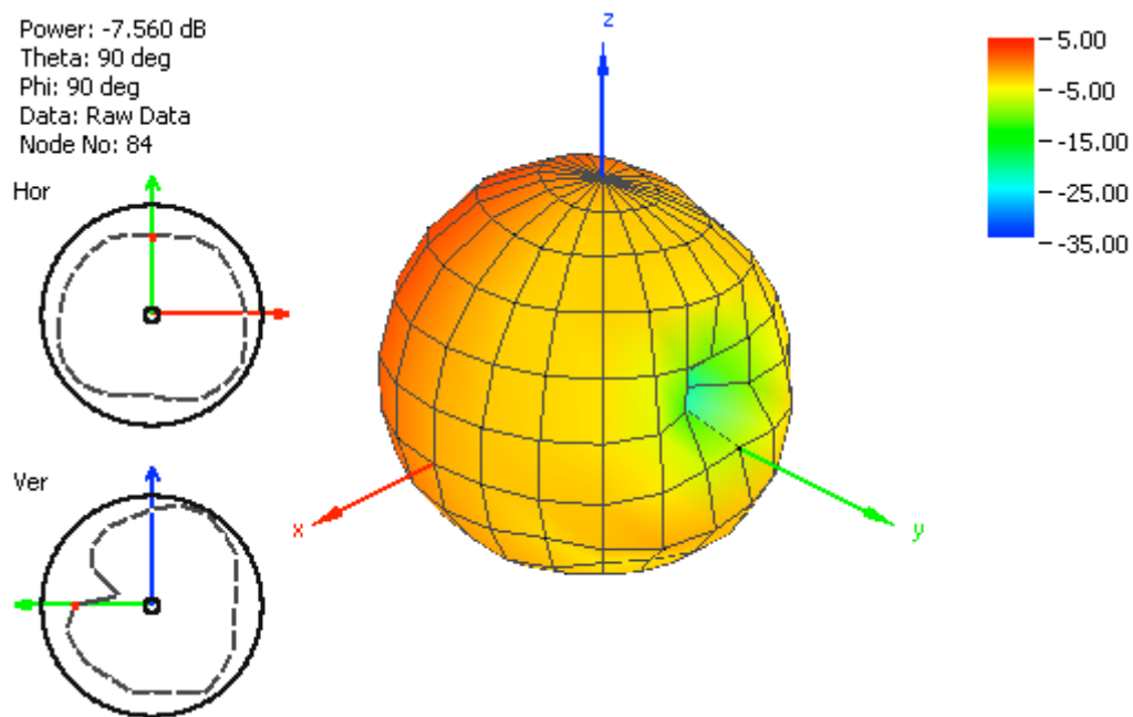
Figure 22. Radiation Pattern at 2500 MHz.
