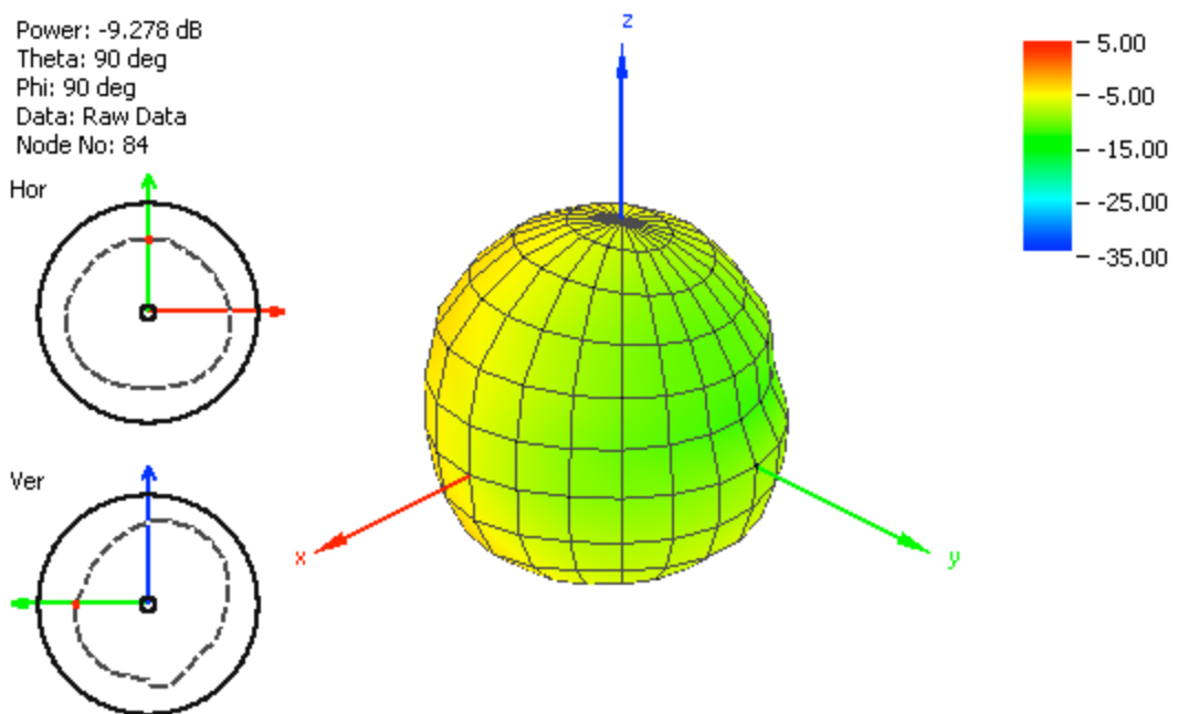
Figure 14. Radiation Pattern at 960 MHz.
