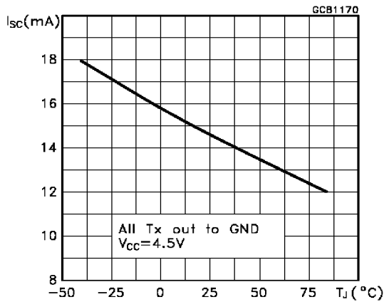
High Level Trasmitter Output Short Circuit Current vs Temperature
