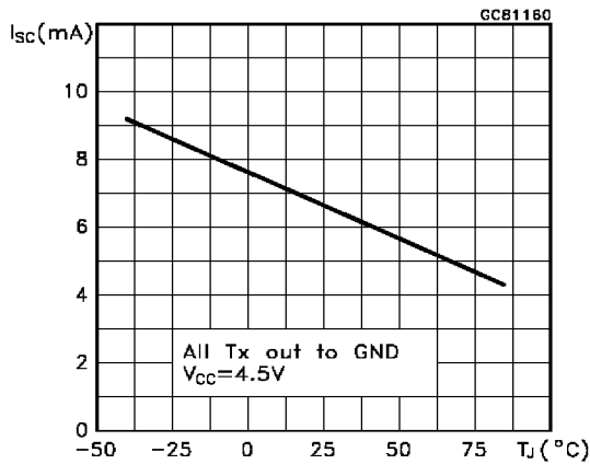
Low Level Trasmitter Output Short Circuit Current vs Temperature
