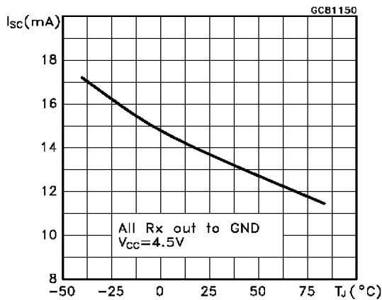
High Level Receiver Output Short Circuit Current vs Temperature
