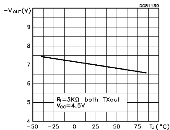
Low Level Output Voltage Swing vs Temperature
