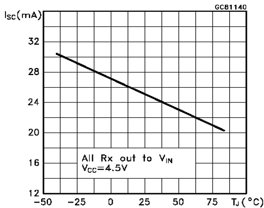
Low Level Receiver Output Short Circuit Current vs Temperature
