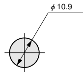
Layout of a Hole for Installation
