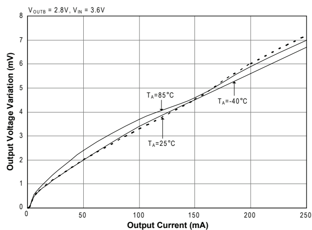
Load Regulation — LDOB
