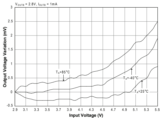
Line Regulation — LDOB
