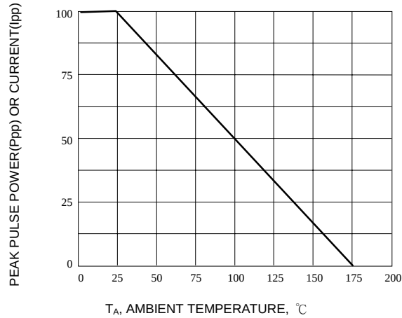
Fig. 2-PULSE DERATING CURVE
