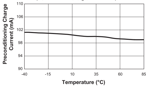
Preconditioning Charge Current vs. Temperature (RSET = 1.58KΩ; ICH_CC = 1000mA)
