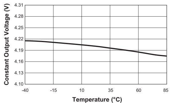
Constant Output Voltage vs. Temperature (RSET = 3.16KΩ; ICH_CC = 500mA)
