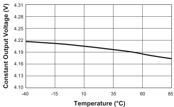
Constant Output Voltage vs. Temperature (RSET = 1.58KΩ; ICH_CC = 1000mA)
