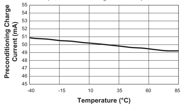
Preconditioning Charge Current vs. Temperature (RSET = 3.16KΩ; ICH_CC = 500mA)
