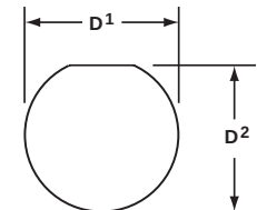
JAM NUT D-HOLE MOUNTING
