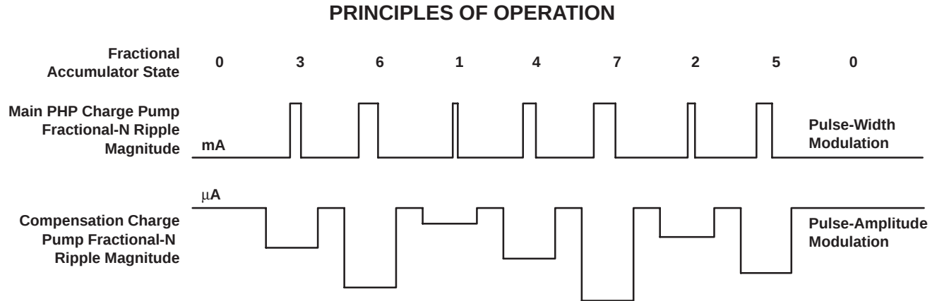
Figure 8. Main PHP and Compensation Charge Pump Fractional-N Waveforms for 3/8 Channel
