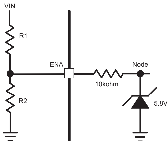
Figure 31. Node Voltage
