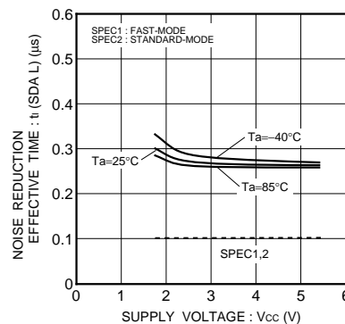
Fig.47 Noise spike width t_i (SDA L)
