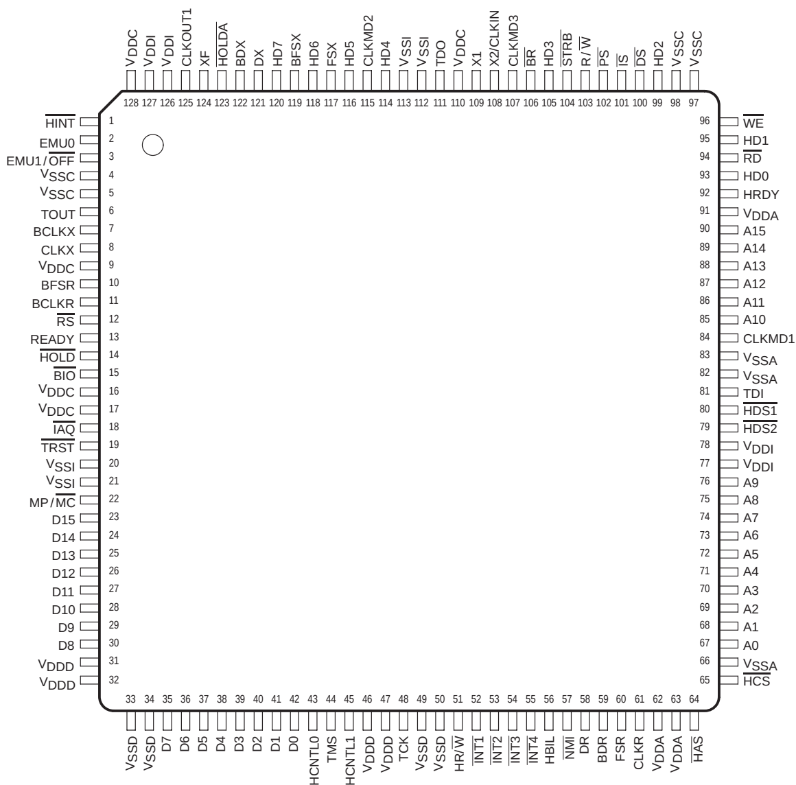
TMS320LC57 PBK PACKAGE ( TOP VIEW )
